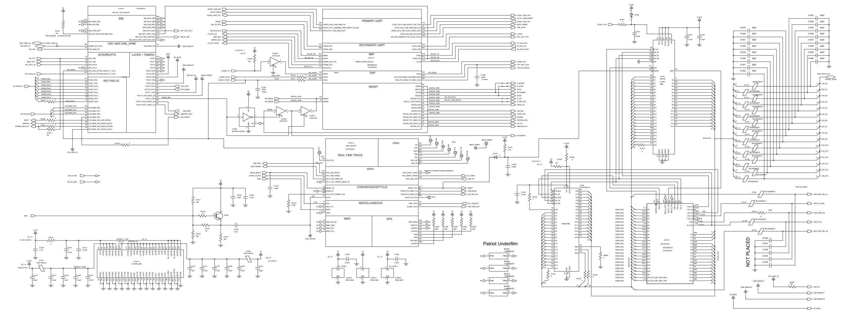
Figure 8-13. VOCON: Controller and Memory Circuits
