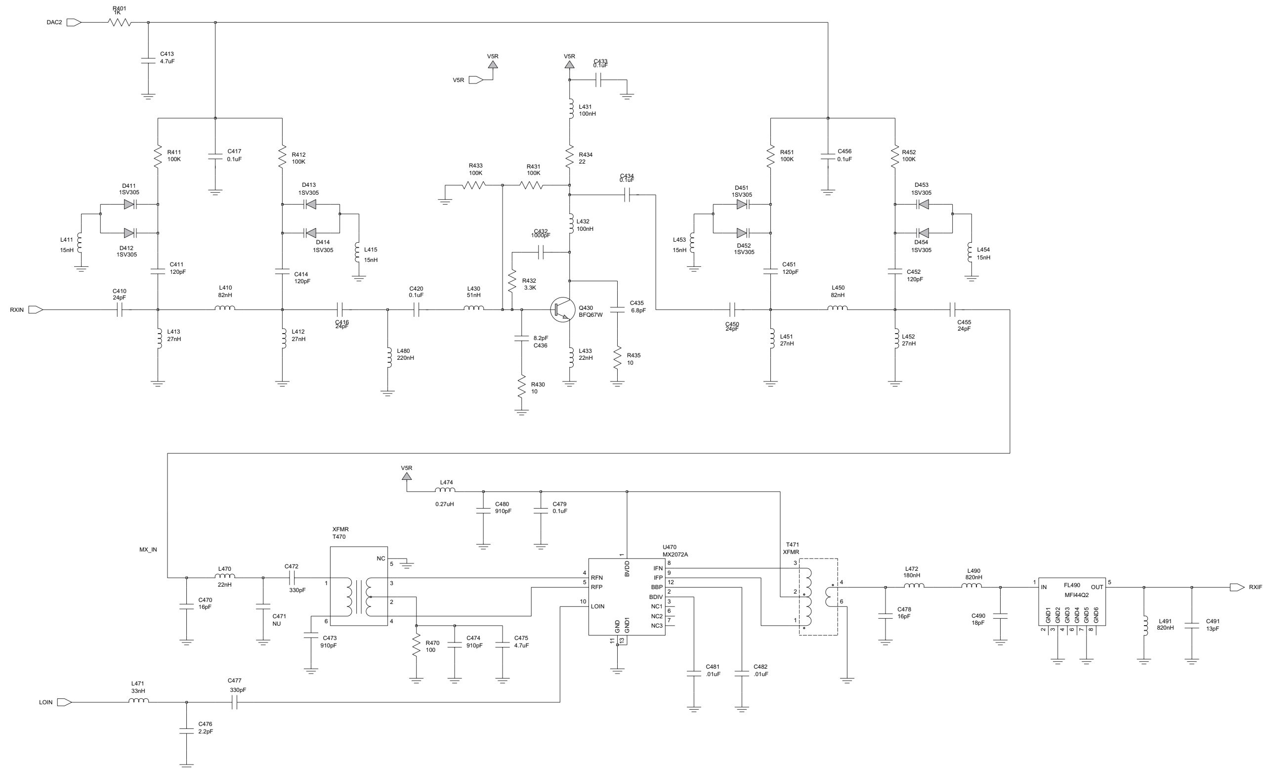
Figure 8-6. VHF Transceiver (RF) Receiver Front End Circuit
