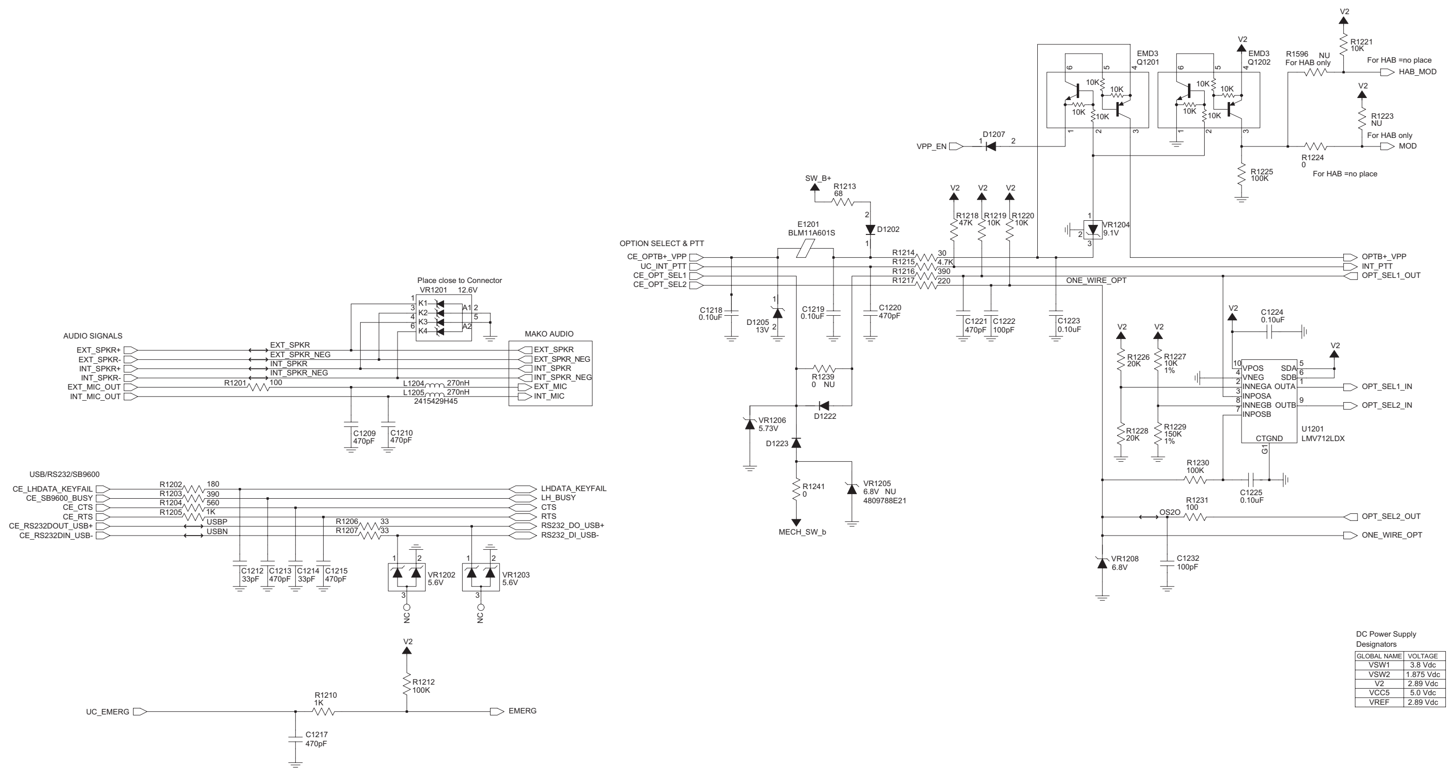
Figure 9-13. VOCON: Audio, Connector Interface Circuits
