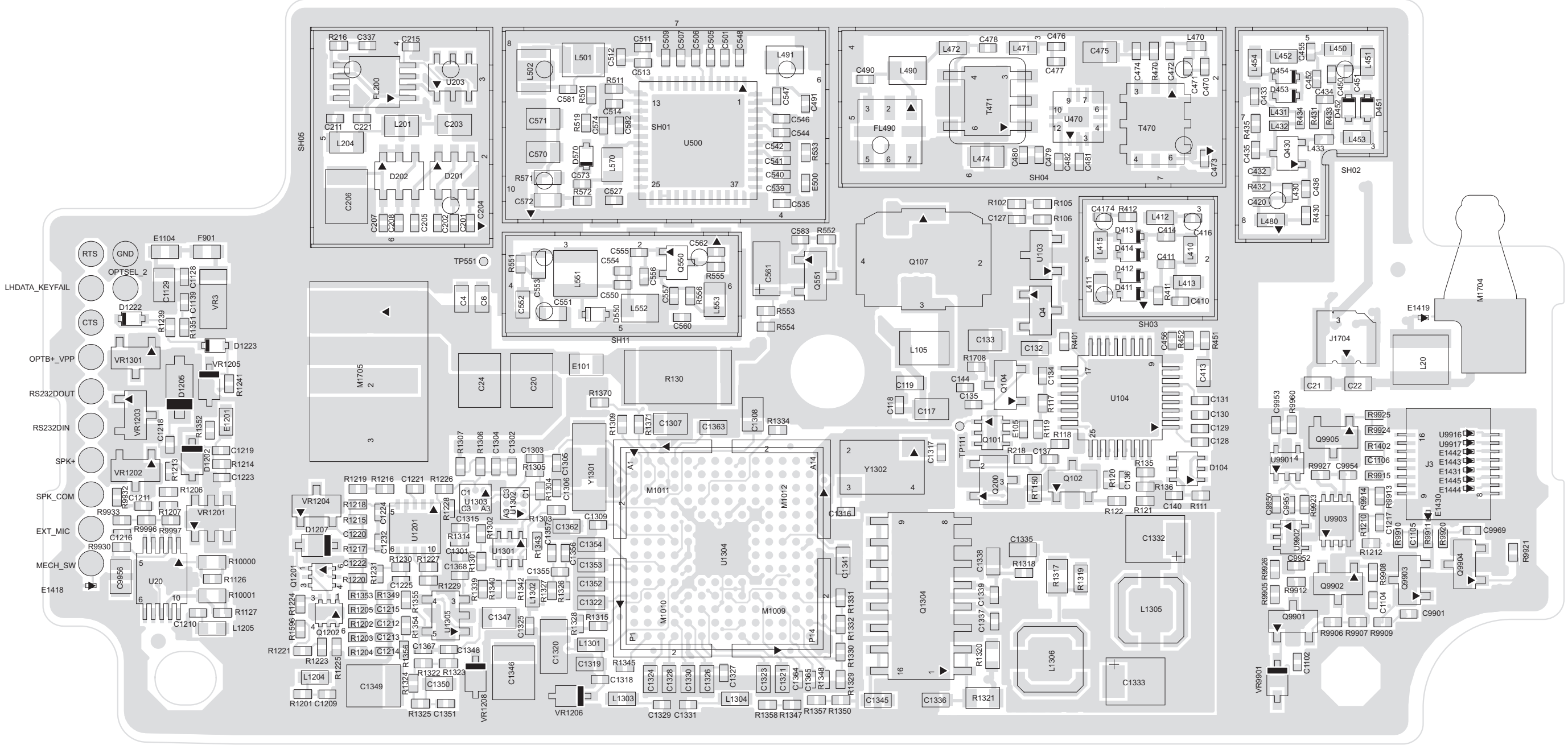
Figure 8-2. Main Board Layout (NUD7115B) – Side 2
