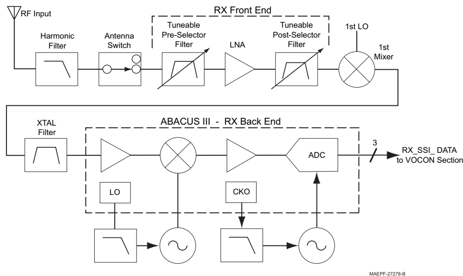
Figure 3-3. Receiver Block Diagram
