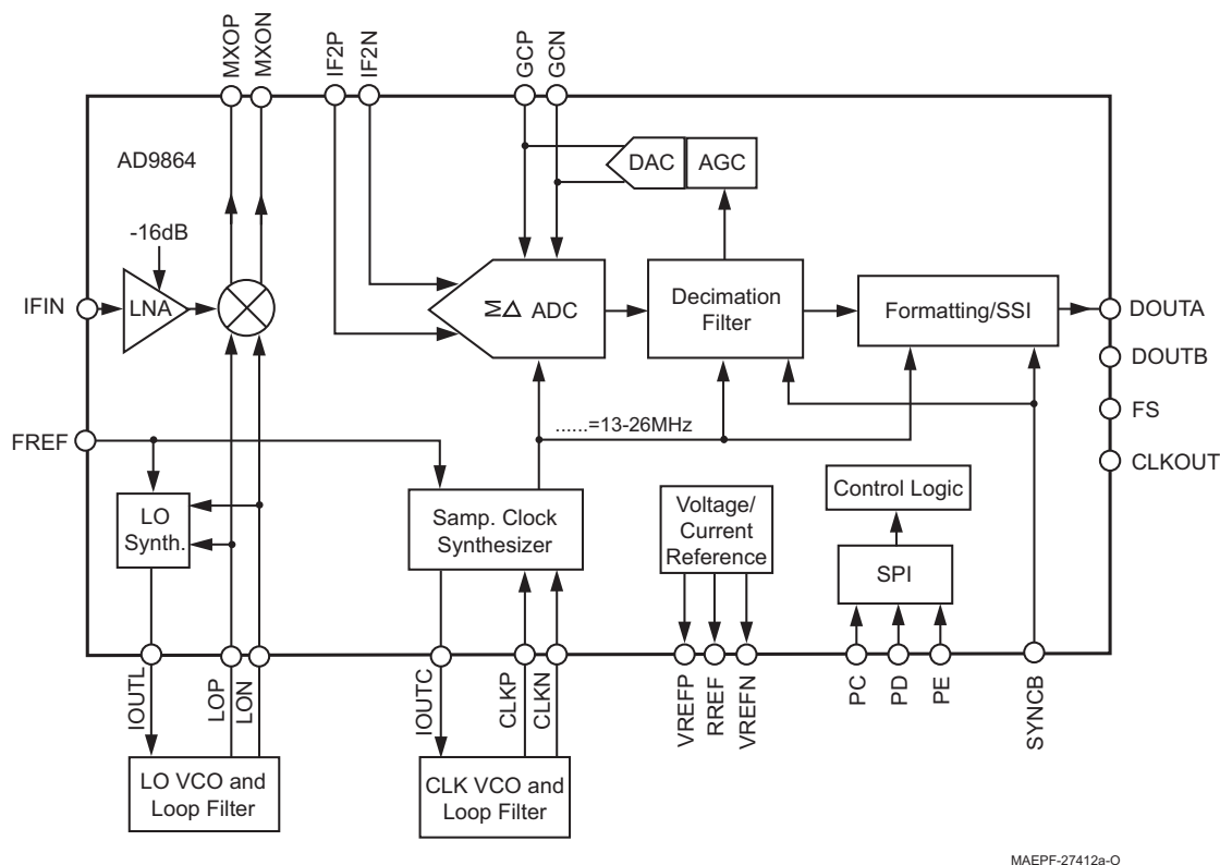
Figure 3-4. Abacus III (AD9864) Functional Block Diagram (from data sheet)
