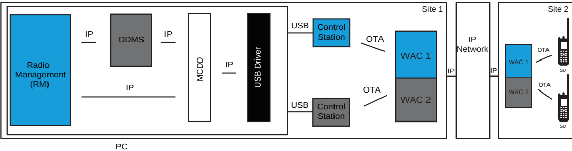
Figure 188: Multi-Channel RM Application with Control Stations in IP Site Connect Mode
