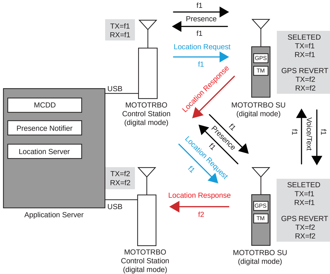
Figure 101: MOTOTRBO Radios in Two Channel Direct Mode GPS Revert Configuration
