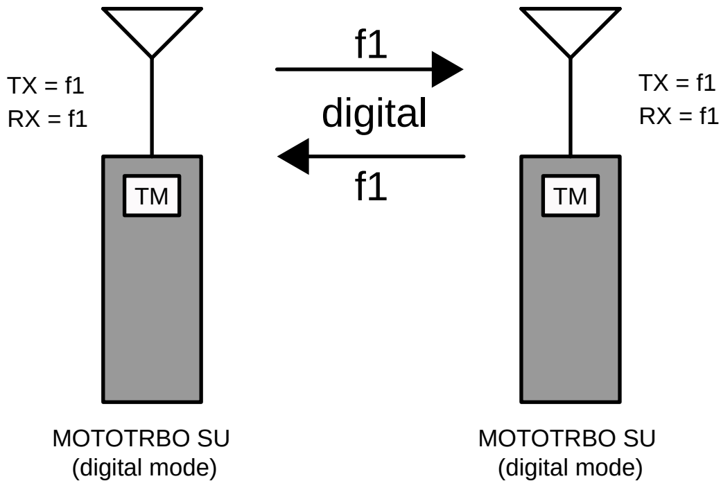
Figure 92: MOTOTRBO Radios (in digital mode) Text Messaging In Direct Mode/Dual Capacity Direct Mode
