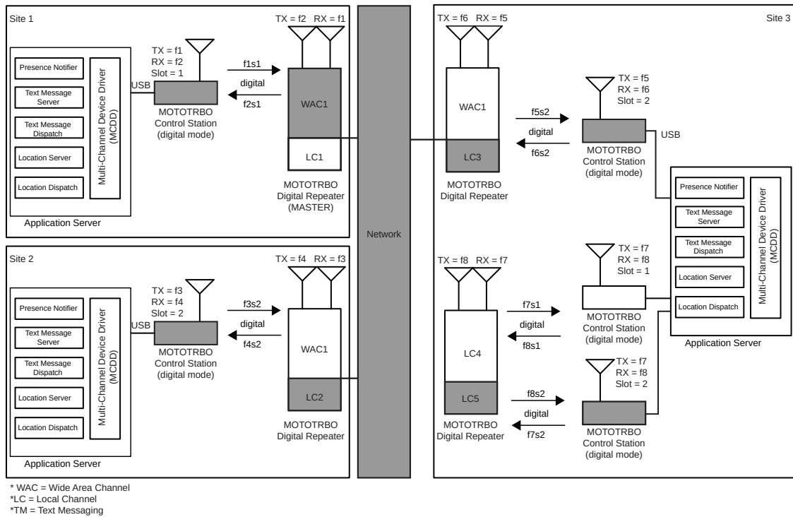
Figure 122: Wide and Local Area System with Distributed Data Application Servers
