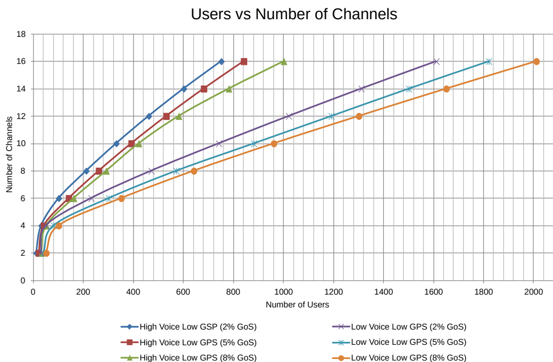
Figure 143: Number of Users Versus Number of Channels for Mixed Profiles
