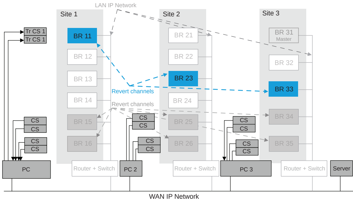
Figure 135: Capacity Plus Multi Site System with Data over Local Revert Channels
