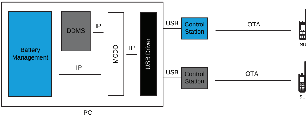
Figure 41: BMA Deployment in Multi-Channel Direct Mode with Control Stations
