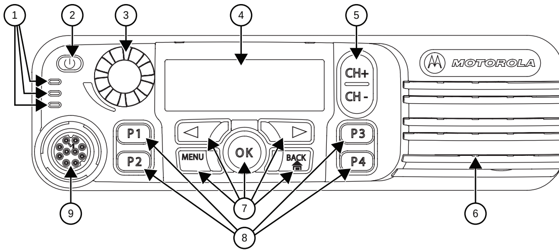
Figure 90: MOTOTRBO Mobile Control Head (Numeric Display Model)
