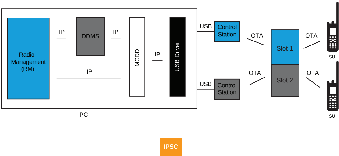
Figure 188: Multi-Channel RM Application with Control Stations in IP Site Connect Mode
