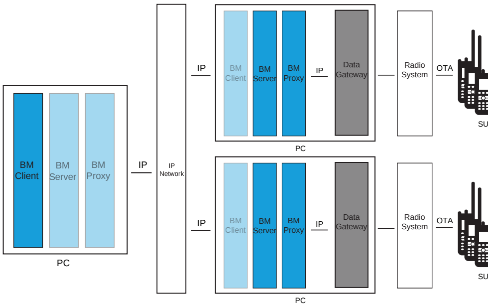
Figure 49: BMA Deployment with Client Remote from Multiple Server and Proxies
