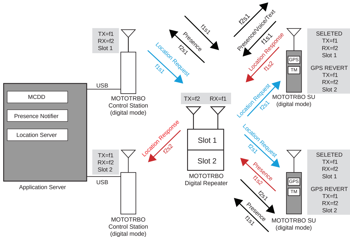
Figure 114: MOTOTRBO Radios in Two-Slot Digital Repeater Mode with GPS Revert Configuration
