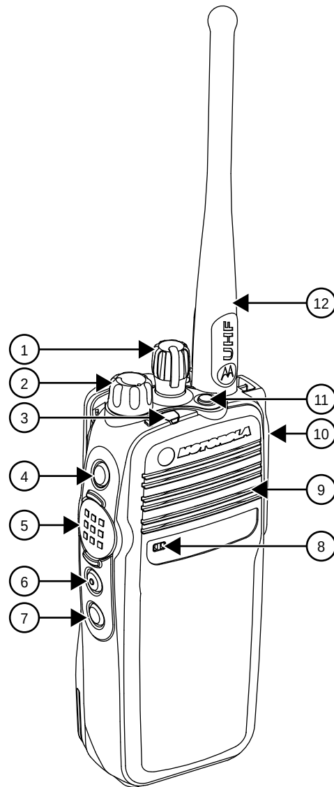
Figure 88: MOTOTRBO Portable (Non-Display Model)
