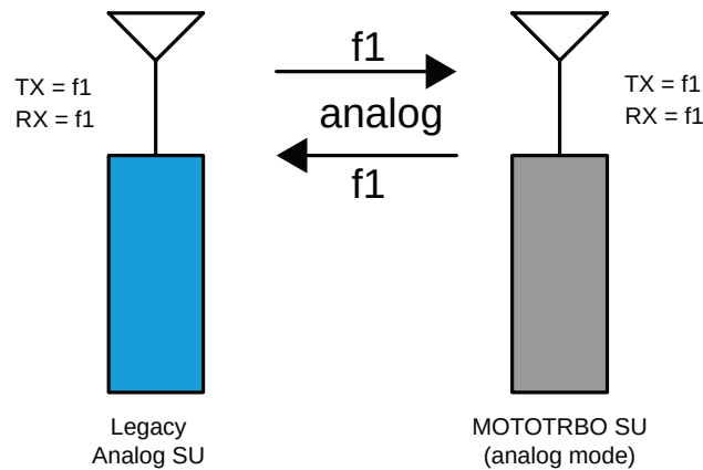
Figure 102: Legacy Analog Radios and MOTOTRBO Radios (in analog mode) in Direct Mode
