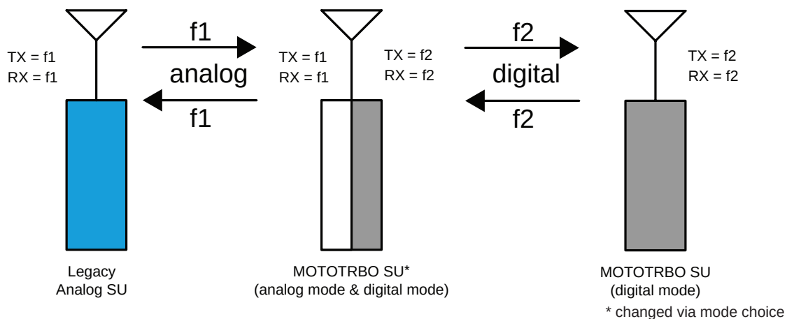
Figure 103: Legacy Analog and MOTOTRBO Analog and Digital Radios in Direct Mode
