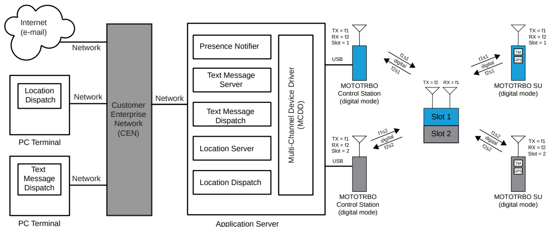
Figure 112: MOTOTRBO Radios in Digital Two-Slot Digital Repeater Mode with a Server-Based Configuration Using Control Stations and Remote Dispatchers
