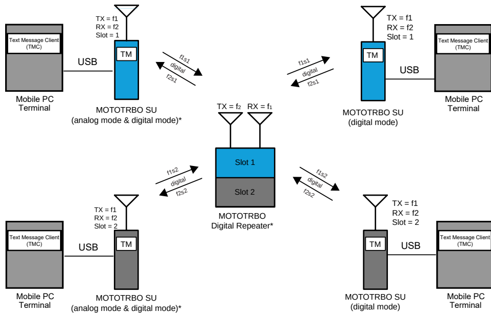
Figure 109: MOTOTRBO Radios in Digital Two-Slot Digital Repeater Mode with Text Messaging
