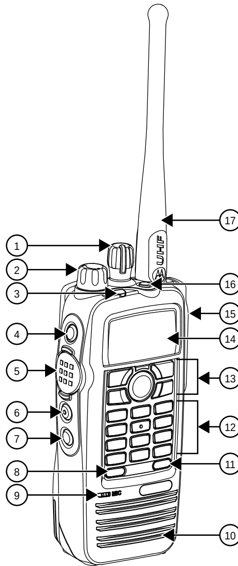
Figure 87: MOTOTRBO Portable (Display Model)
