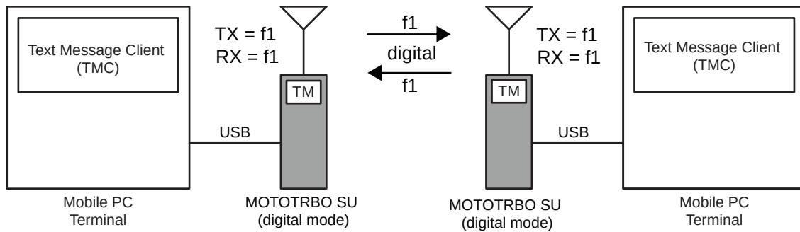
Figure 93: MOTOTRBO Radios (in digital mode) Text Messaging In Multiple Direct Mode/Dual Capacity Direct Mode
