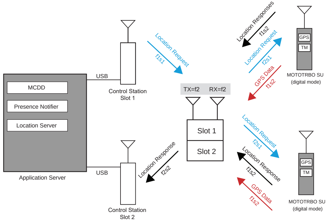
Figure 115: Single Site Conventional System with an Enhanced GPS Revert Channel
