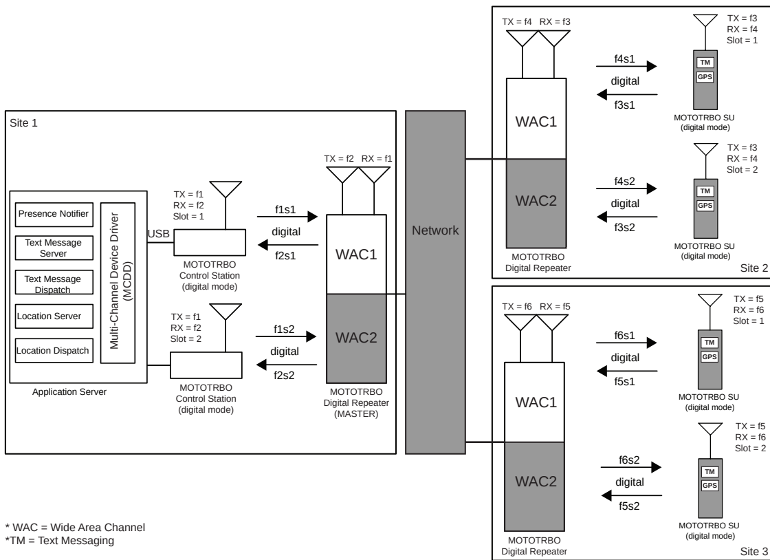
Figure 121: Wide Area System with Centralized Data Application Server
