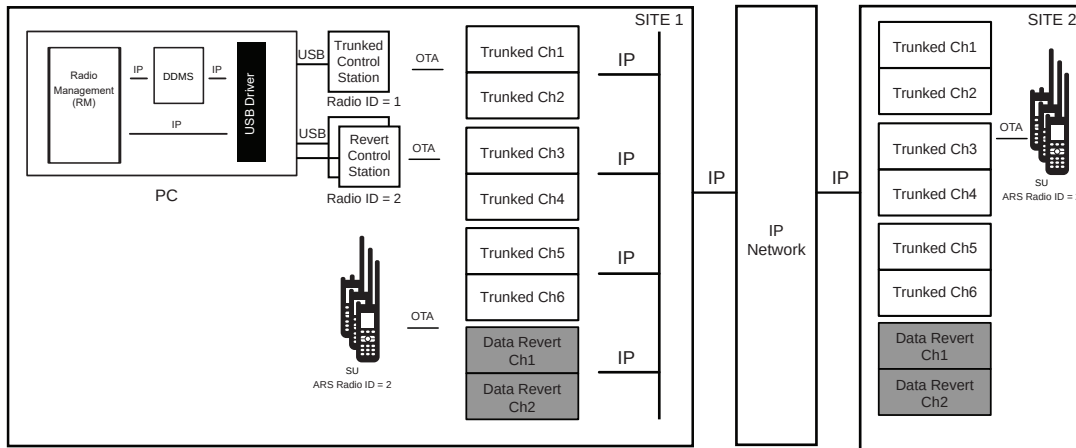
Figure 203: RM Application with Control Stations in a Capacity Plus Multi Site System with Presence (DDMS) and Wide Area Data Revert Channels
