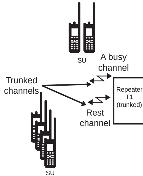
Figure 128: 2-Channel Capacity Plus Single Site System without Data Application Server
