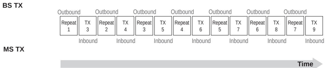
Figure 106: Time Division Duplex Repeater
