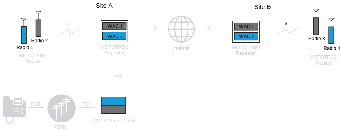
Figure 67: Two APP Boxes Supporting Two Wide Area Channels in IP Site Connect
