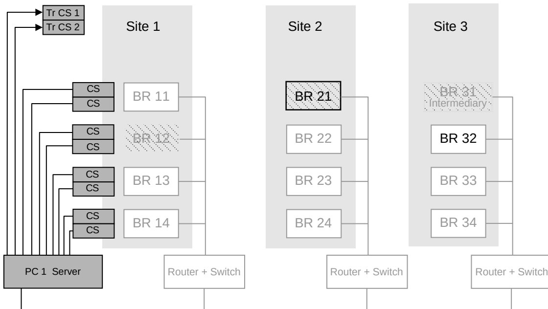
Figure 134: Capacity Plus Multi Site System with Data over Trunked Channels
