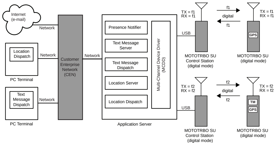
Figure 100: MOTOTRBO Radios in Two Channel Digital Direct Mode Server-Based Configuration with Remote Dispatchers
