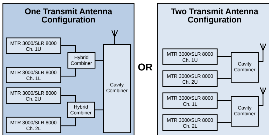
Figure 80: RF Site Configurations for MOTOTRBO 2-4-1 Channels
