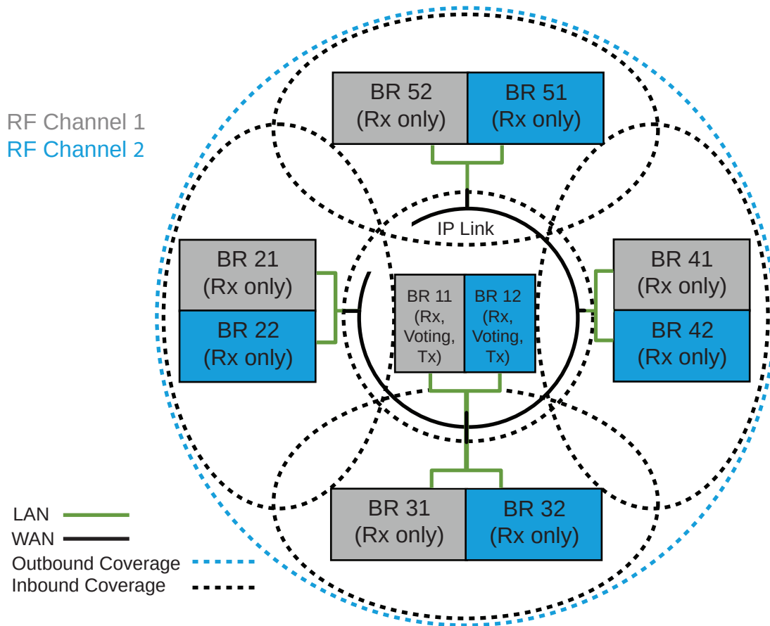
Figure 139: Digital Voting Topology for a Capacity Plus Single Site System
