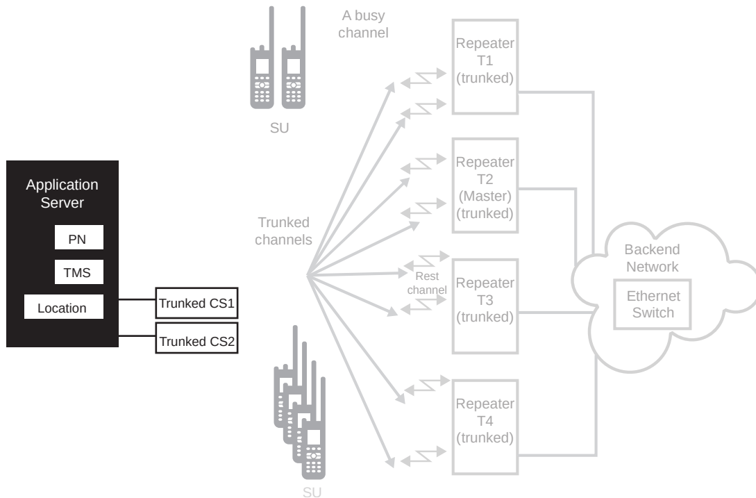
Figure 130: Capacity Plus Single Site Devices with Data over Trunked Channels
