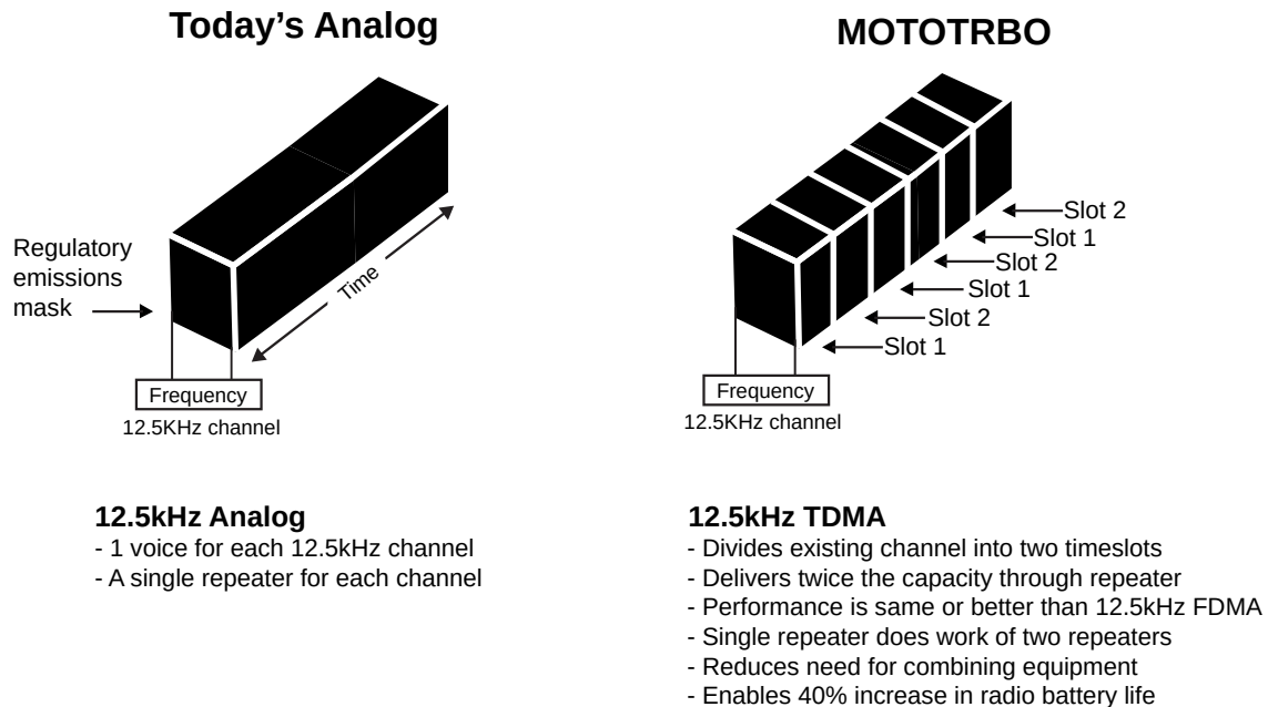
Figure 3: Comparison between Today's Analog and MOTOTRBO
