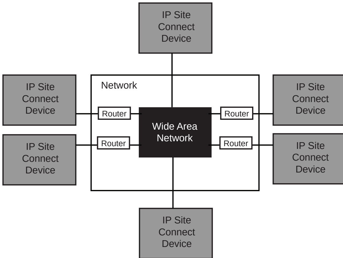
Figure 125: IP Site Connect Devices connected through Wide Area Network
