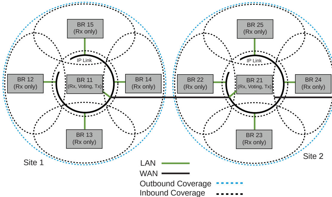
Figure 138: Digital Voting Topology for a Two-Site IP Site Connect System
