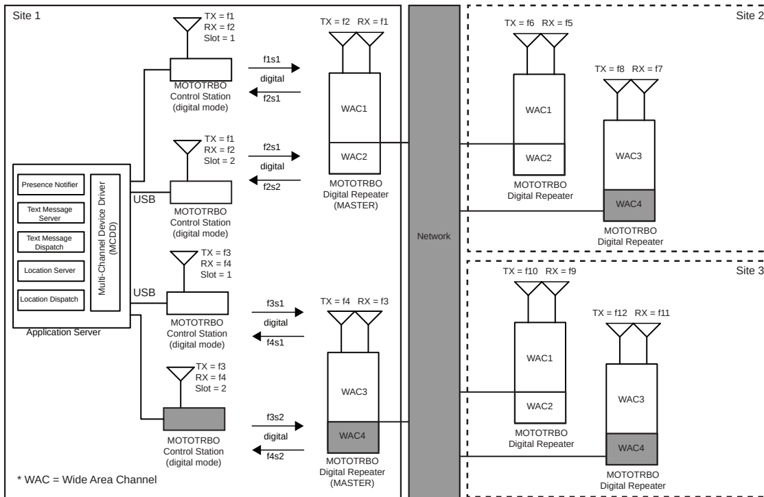
Figure 123: Multiple Wide Area Systems with Centralized Data Application Server
