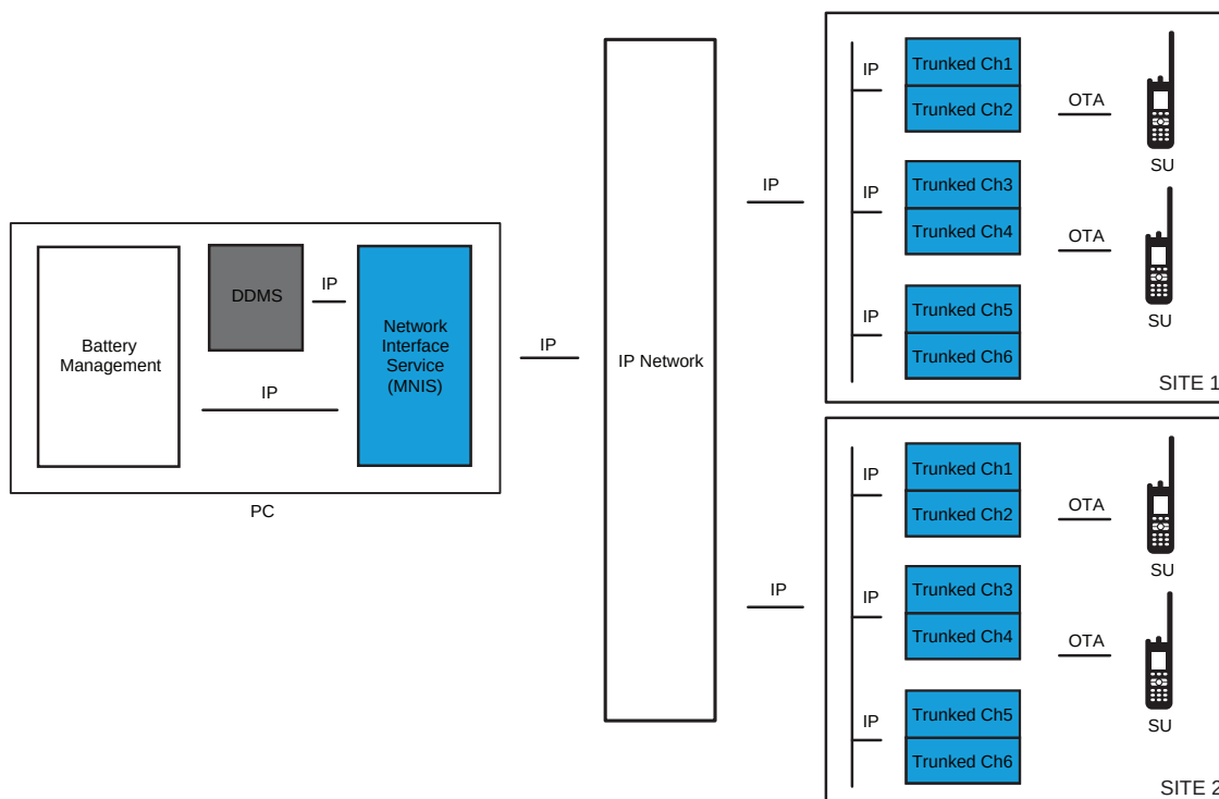
Figure 39: BMA Deployment in Capacity Plus Multi Site with MNIS
