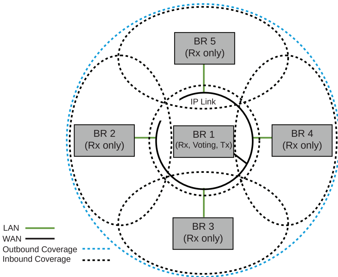
Figure 137: Digital Voting Topology for Conventional Single Site or IP Site Connect Local Channel
