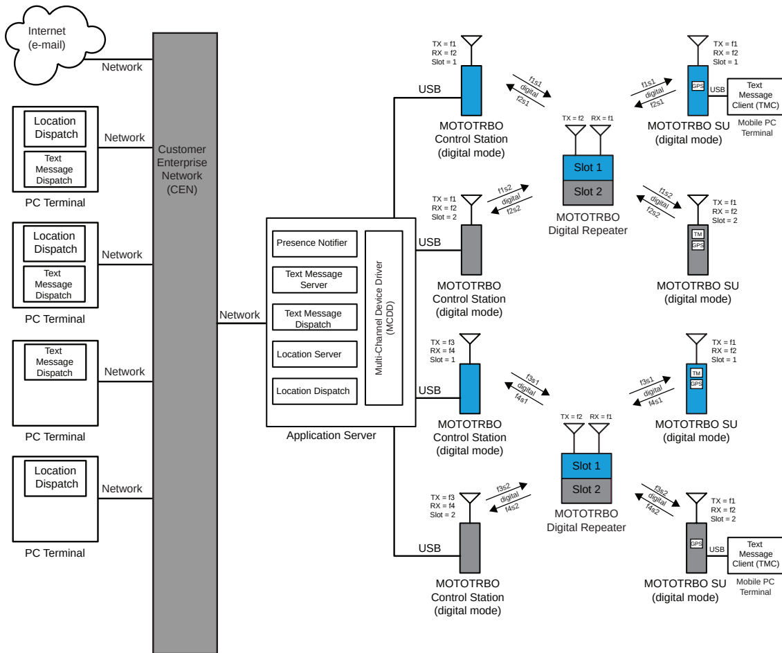
Figure 113: MOTOTRBO Radios in Digital Two-Slot, Digital Repeater Mode with Text Message Server, Location Server Using Control Stations with Local and Remote Dispatchers
