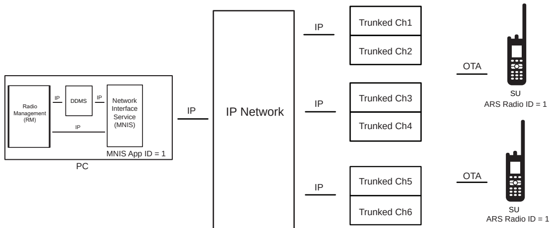
Figure 201: RM Application in a Capacity Plus System with a MNIS and a DDMS
