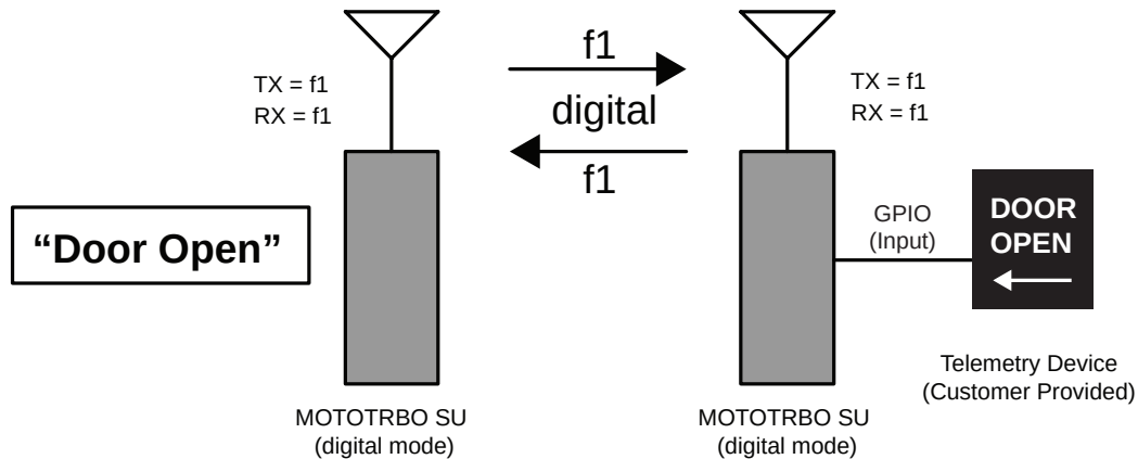
Figure 95: Send Telemetry Message from MOTOTRBO Radio to Another MOTOTRBO Radio when Input Pin State Changes
