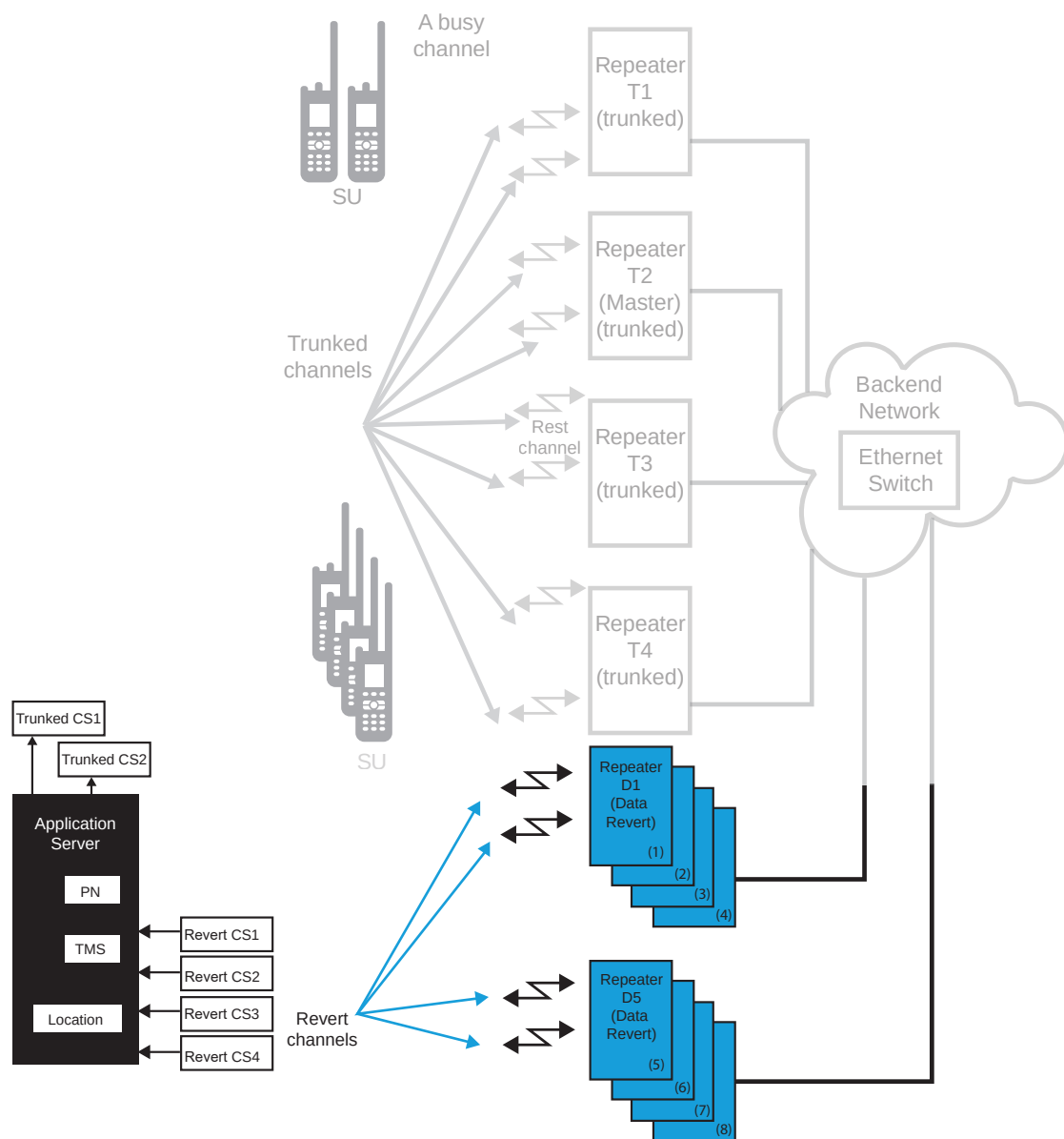
Figure 132: Capacity Plus Single Site Devices with Data over Revert Channels
