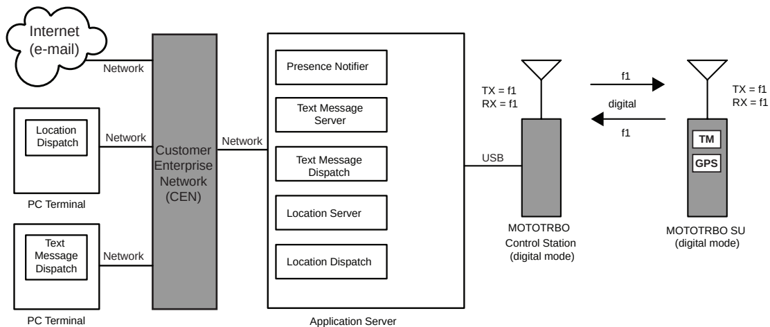
Figure 99: MOTOTRBO Radios In Digital Direct Mode/Dual Capacity Direct Mode Server Based Configuration with Remote Dispatchers
