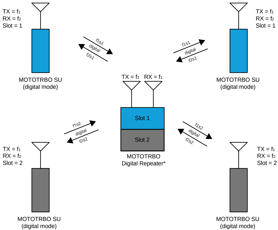
Figure 107: MOTOTRBO Digital Radios on MOTOTRBO Two-Slot Digital Repeater
