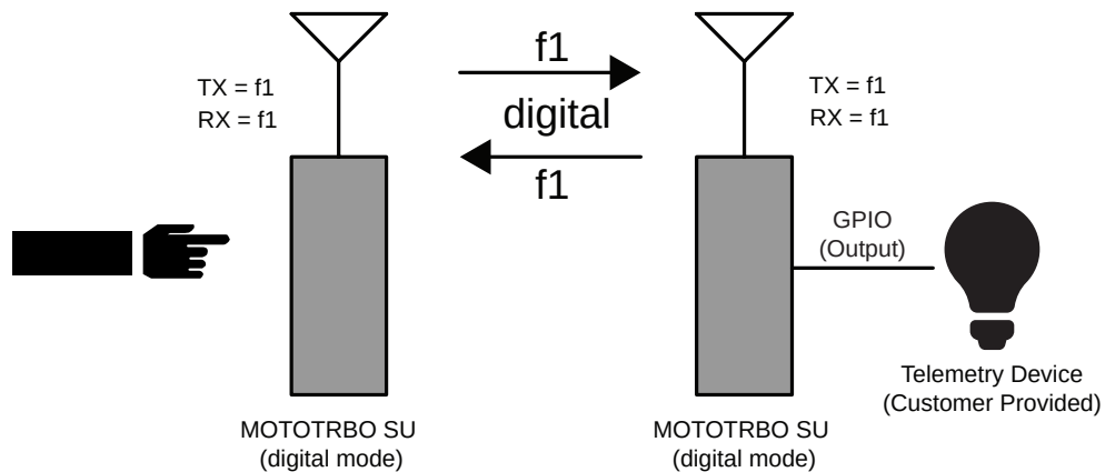
Figure 94: Send Telemetry Command from MOTOTRBO Radio to Another MOTOTRBO Radio to Toggle an Output Pin
