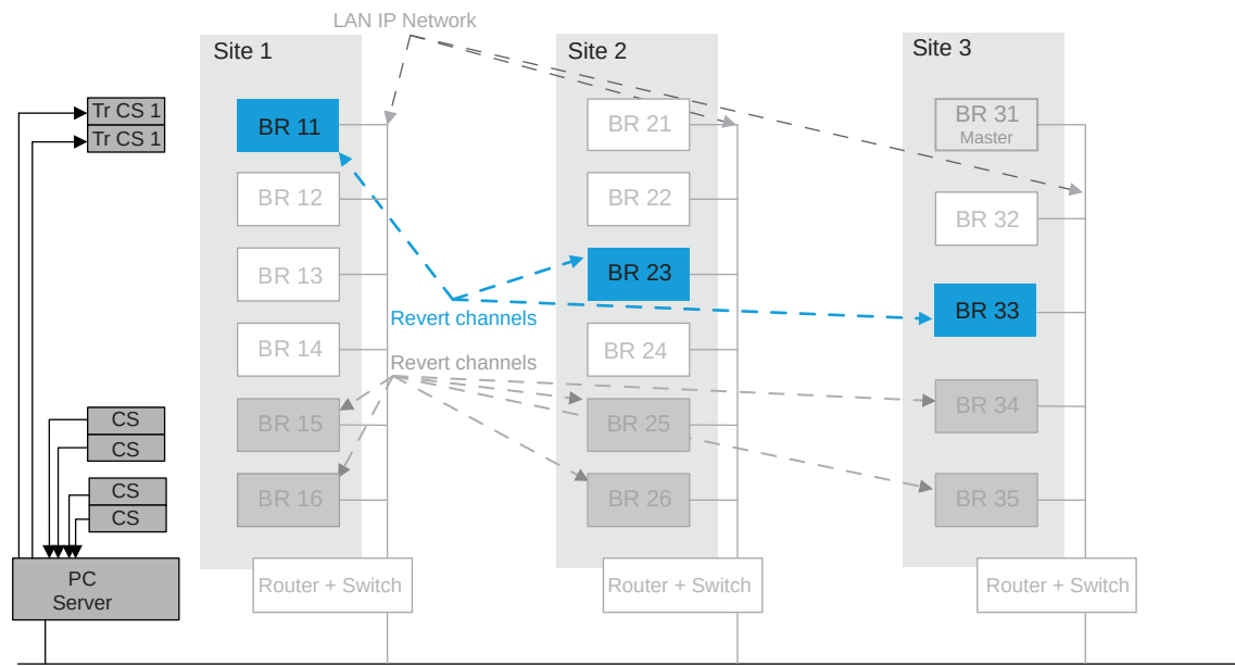
Figure 136: Capacity Plus Multi Site System with Data over Wide Area Revert Channels
