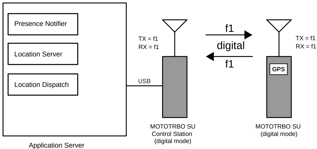
Figure 97: MOTOTRBO Radios In Digital Direct Mode/Dual Capacity Direct Mode with Location Server and Local Location Client
