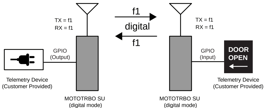
Figure 96: Send Telemetry Command to Toggle an Output Pin from MOTOTRBO Radio to Another MOTOTRBO Radio when Input Pin State Changes
