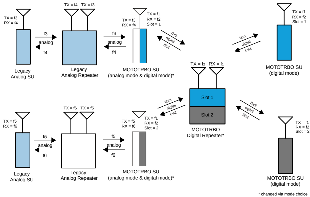
Figure 120: MOTOTRBO Digital Radios on a Two-Slot MOTOTRBO Digital Repeater with Analog Repeater Support
