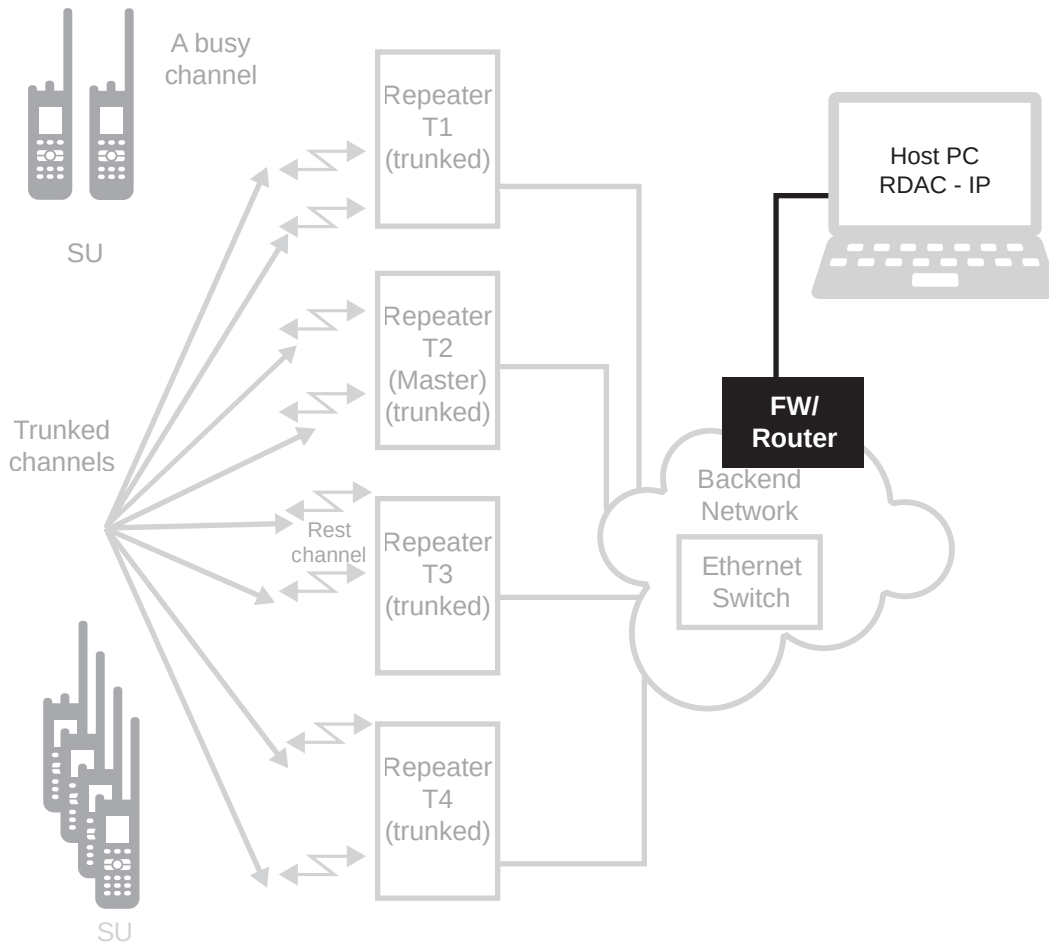
Figure 129: Capacity Plus Single Site Devices with Remote RDAC and no Data Application Server
