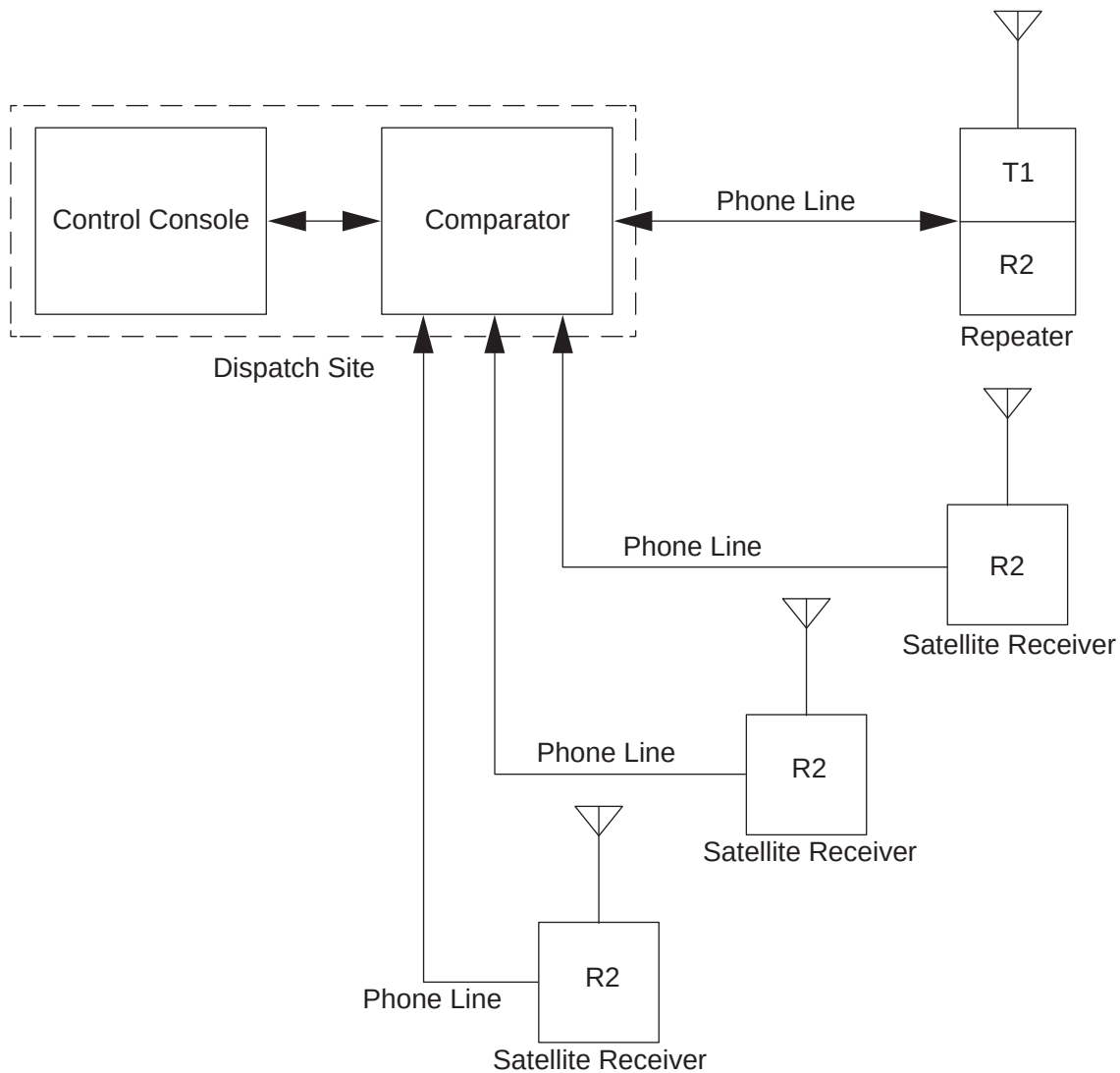
Figure 82: Satellite Receiver Connections Within a Voting System
