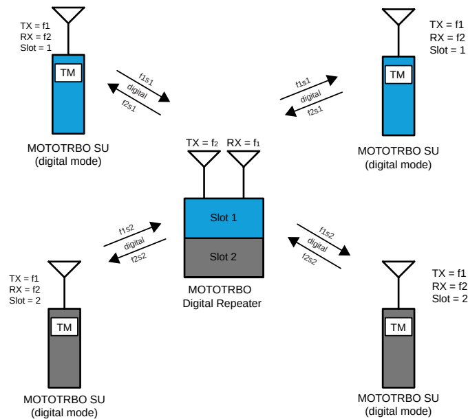
Figure 108: MOTOTRBO Radios in Digital Two-Slot Digital Repeater Mode with Built-In Text Messaging
