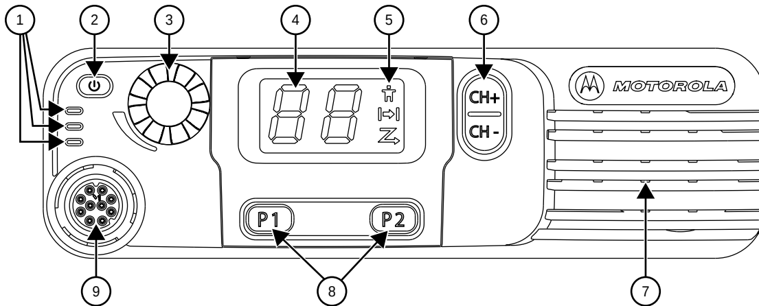
Figure 90: MOTOTRBO Mobile Control Head (Numeric Display Model)
