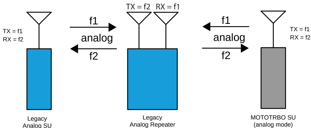
Figure 118: MOTOTRBO Analog and Legacy Analog Radios on Legacy Analog Repeater
