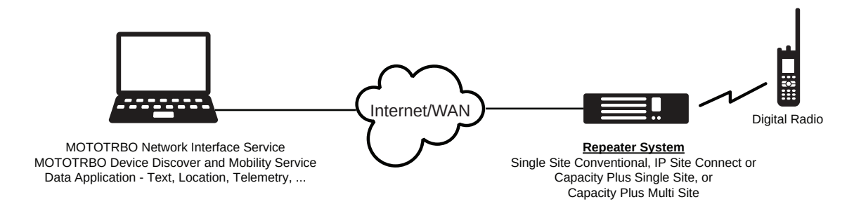
Figure 86: MOTOTRBO Network Interface Service (MNIS)
