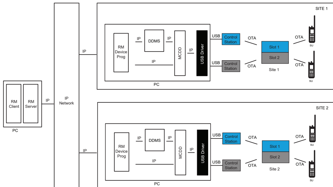
Figure 191: RM Application with Control Stations Covering RF Isolated Single Site Repeaters Using Remote Device Programmers
