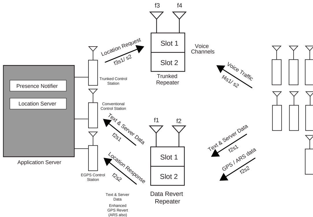
Figure 117: A Capacity Plus Single Site System with an Enhanced GPS Revert Channel
