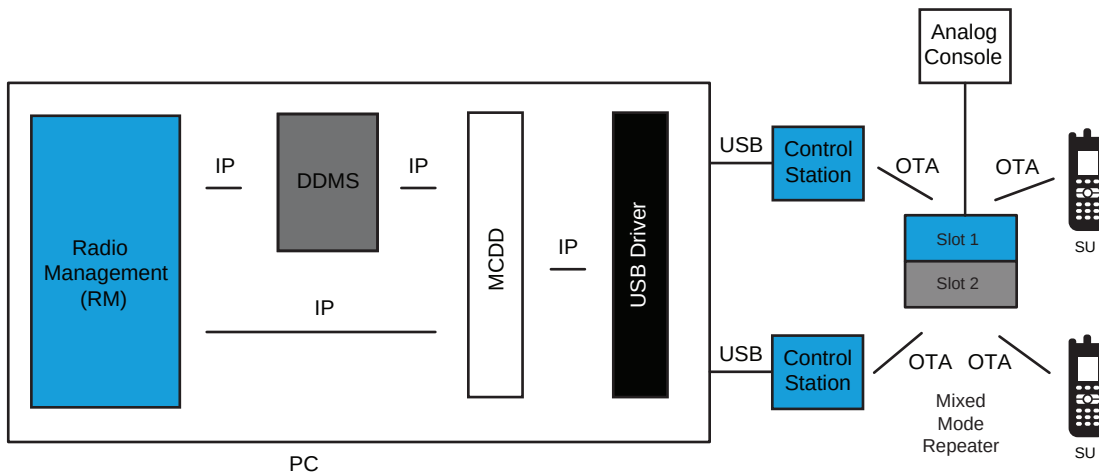
Figure 195: RM Application in Dynamic Mixed Mode
