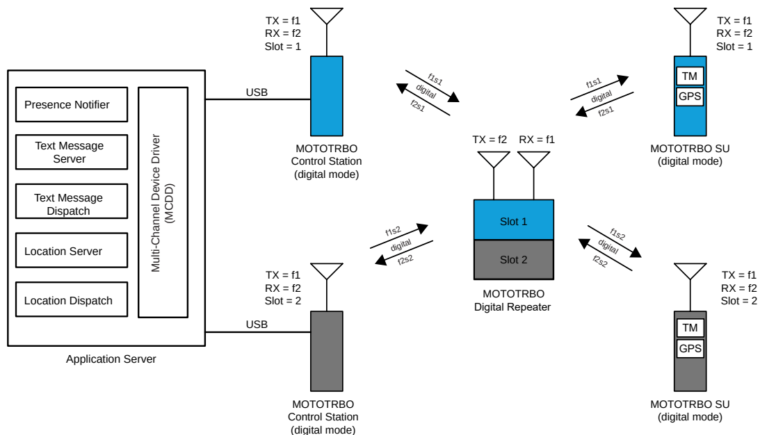
Figure 111: MOTOTRBO Radios in Digital Two-Slot Digital Repeater Mode with a Server-Based Configuration Using Control Stations
