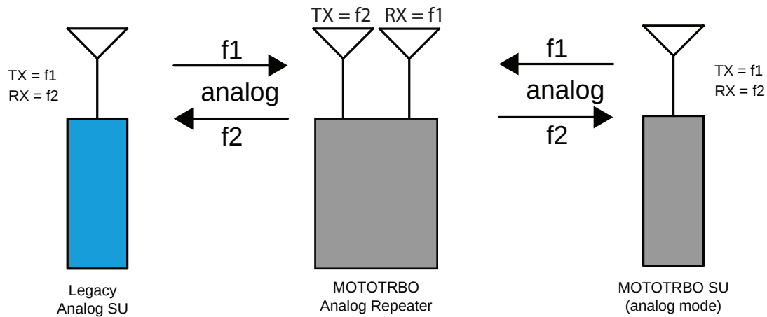
Figure 119: MOTOTRBO Analog and Legacy Analog Radios on MOTOTRBO Analog Repeater
