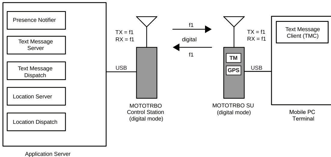
Figure 98: MOTOTRBO Radios In Digital Direct Mode with Text Message Server, Location Server and Local Dispatchers
