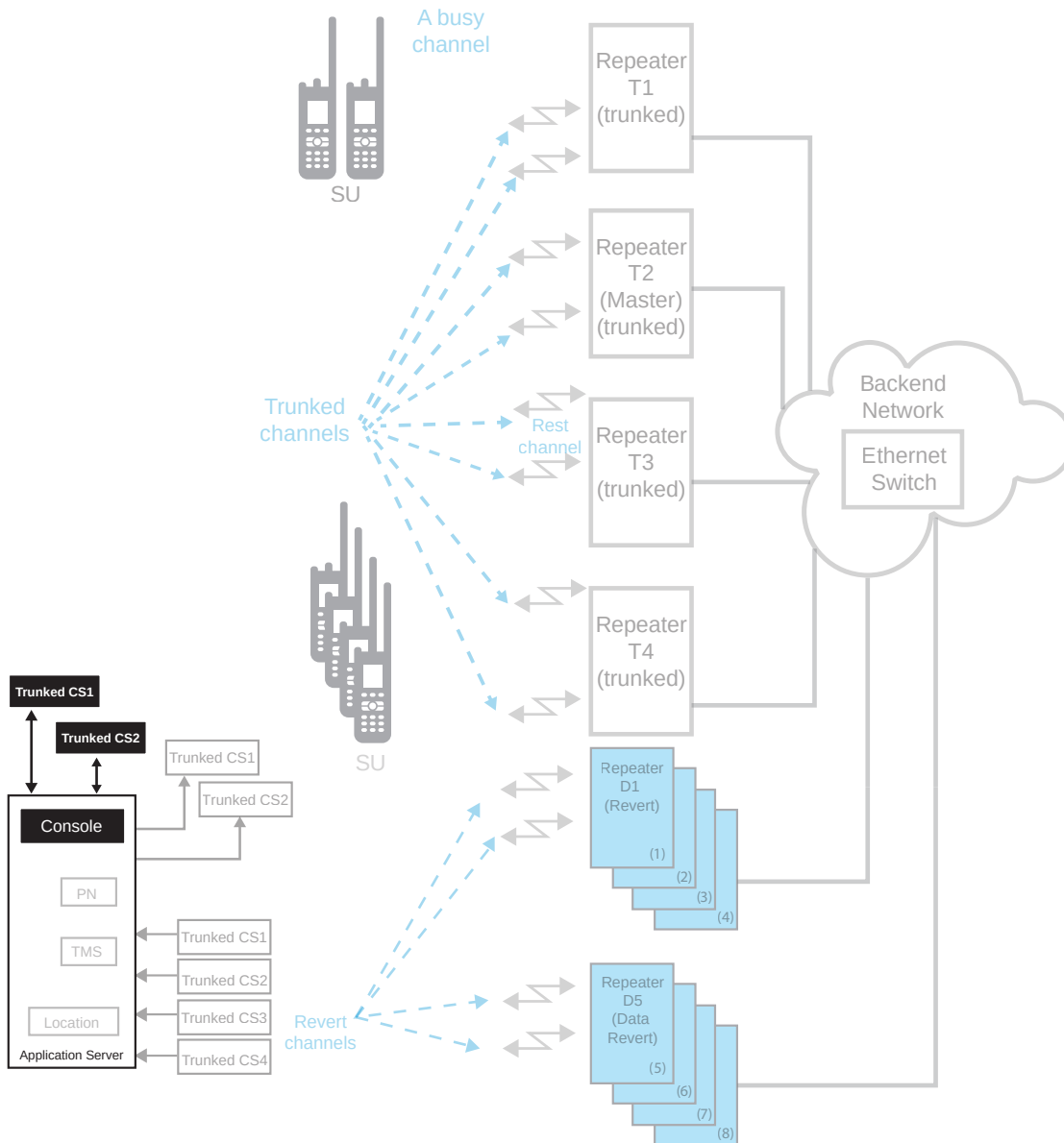
Figure 133: Capacity Plus Single Site Devices with a Dispatch Station (Console)
