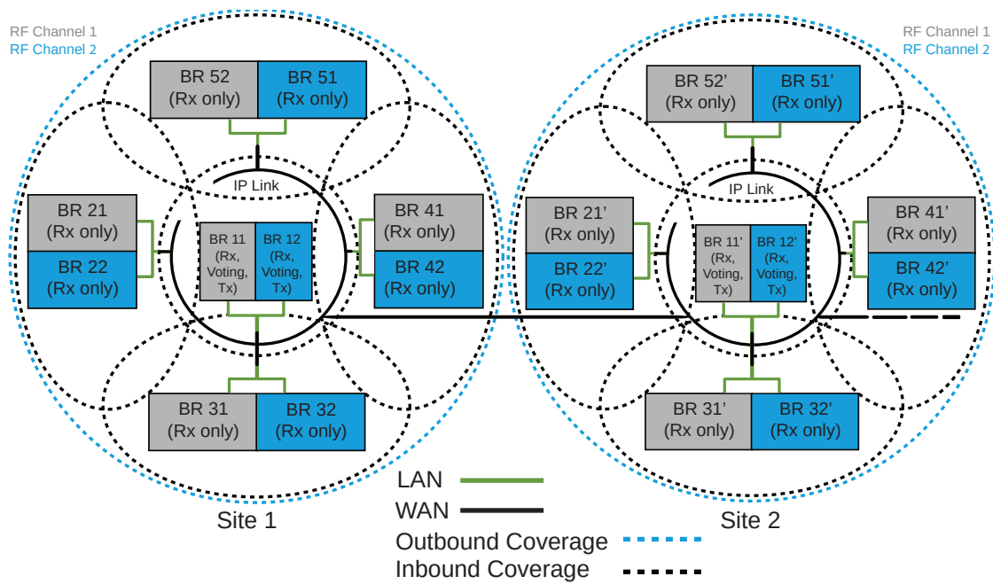
Figure 140: Digital Voting Topology for a 2-Site Capacity Plus Multi Site System
