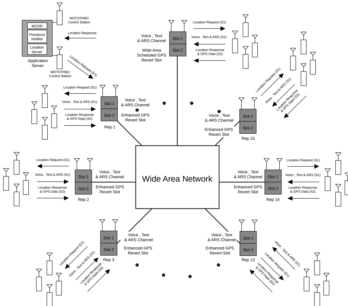
Figure 116: IP Site Connect System with an Enhanced GPS Revert Channel
