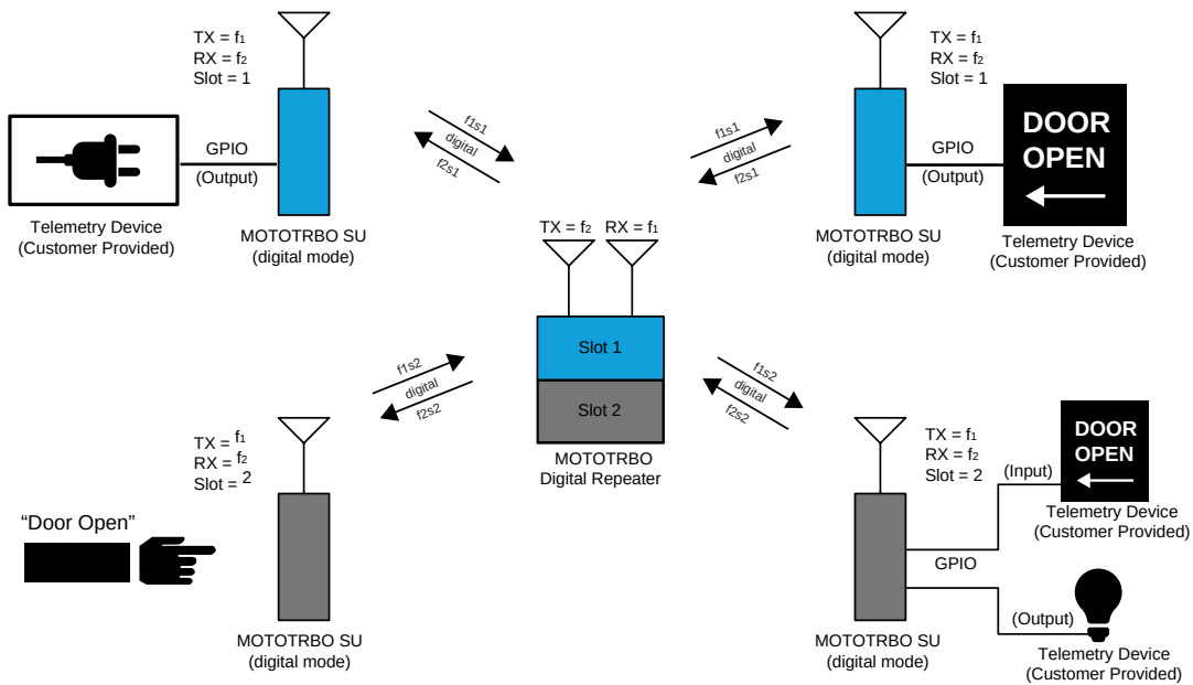
Figure 110: MOTOTRBO Radios in Digital Two-Slot Digital Repeater Mode with Telemetry Functions
