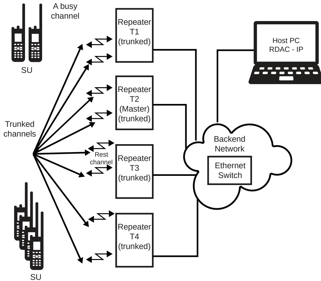
Figure 127: Capacity Plus Single Site Devices with Local RDAC and no Data Application Server
