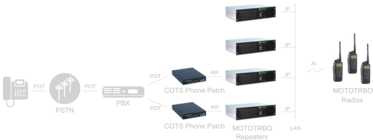
Figure 2-25 Phone Patch Topology in a Capacity Plus Configuration
