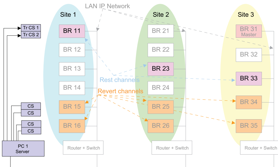
Figure 3-48 A Linked Capacity Plus System with Data over Wide Area Revert Channels
