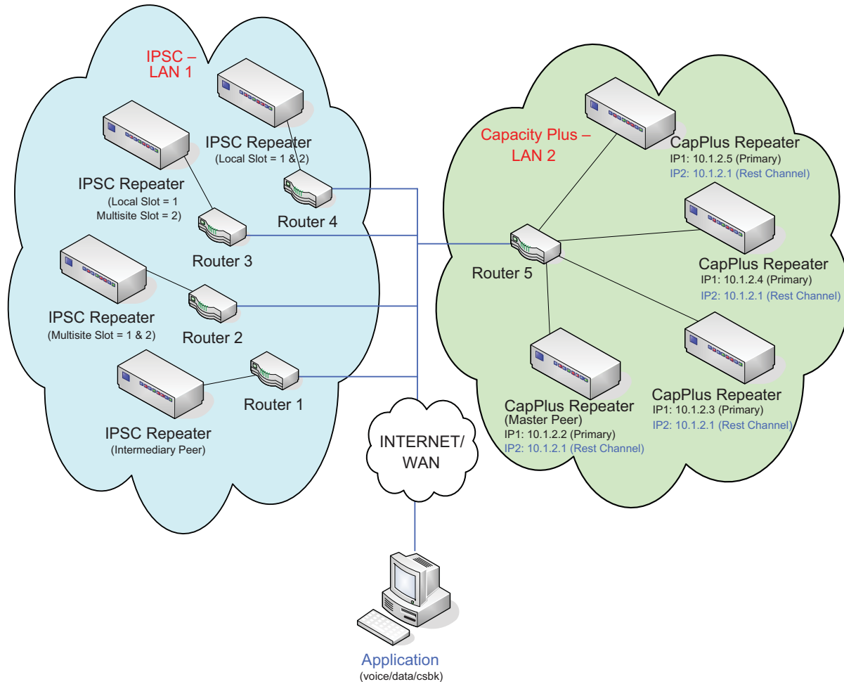
Figure 2-29 Capacity Plus and IP Site Connect System with IP-based ADP Application
