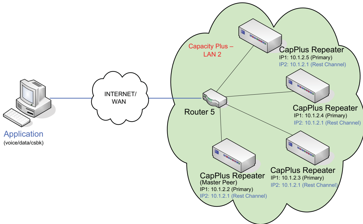
Figure 2-28 Capacity Plus System with IP-based ADP Application
