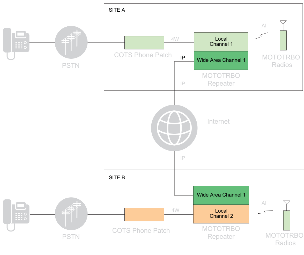
Figure 2-21 Phone Patch Topology in IP Site Connect Local Area Channel Configuration
