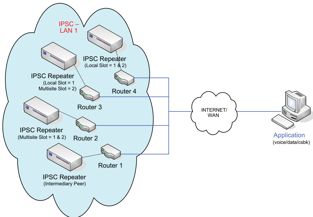
Figure 2-27 IP Site Connect System with IP-based ADP Application
