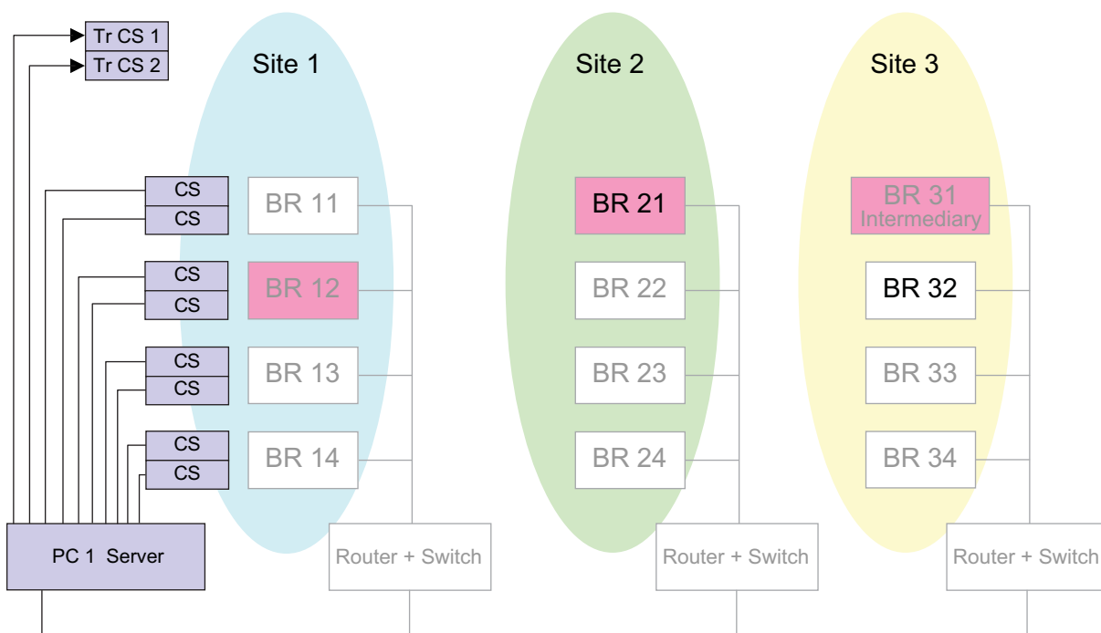
Figure 3-46 A Linked Capacity Plus System with Data over Trunked Channels
