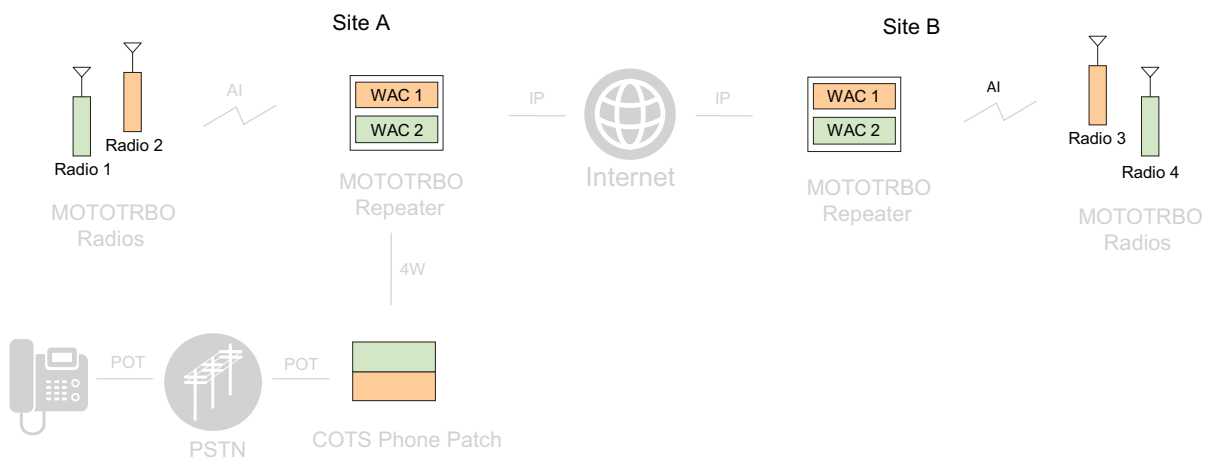
Figure 2-22 One APP Box Supporting Two Wide Area Channels in IP Site Connect
