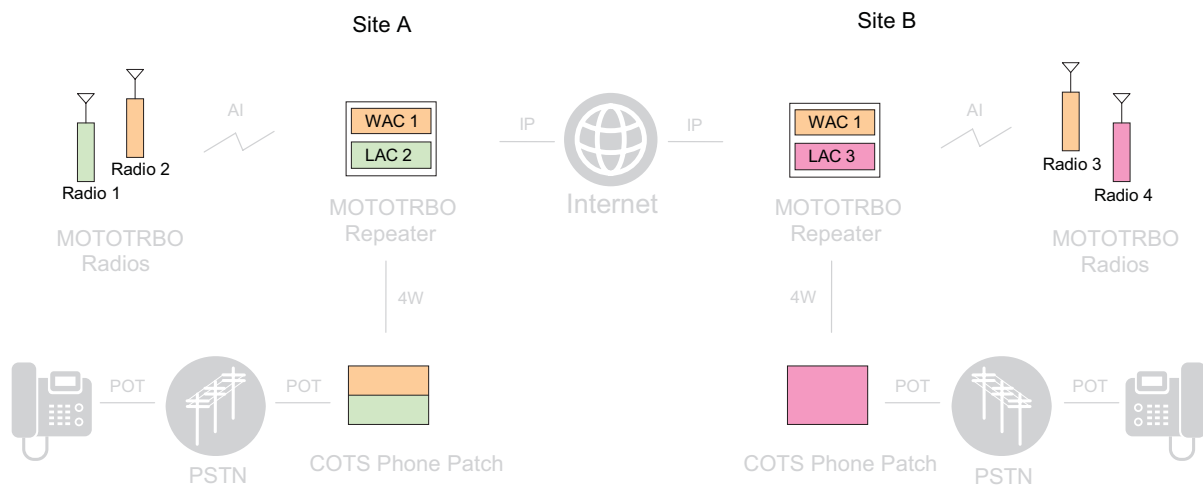
Figure 2-24 APP Boxes Supporting Wide Area Channels and Local Area Channels in IP Site Connect
