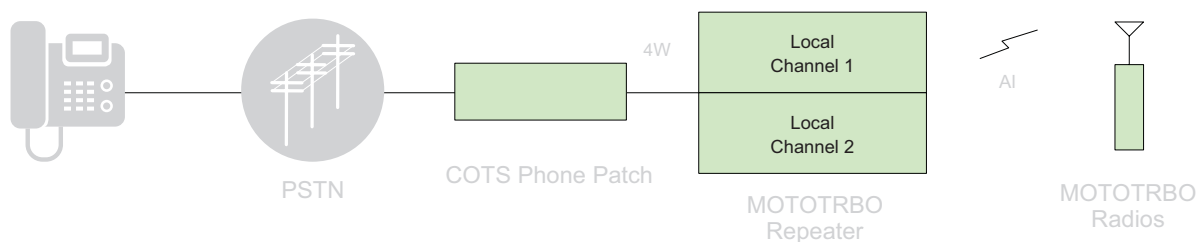
Figure 2-20 Phone Patch Topology in Single Site Configuration
