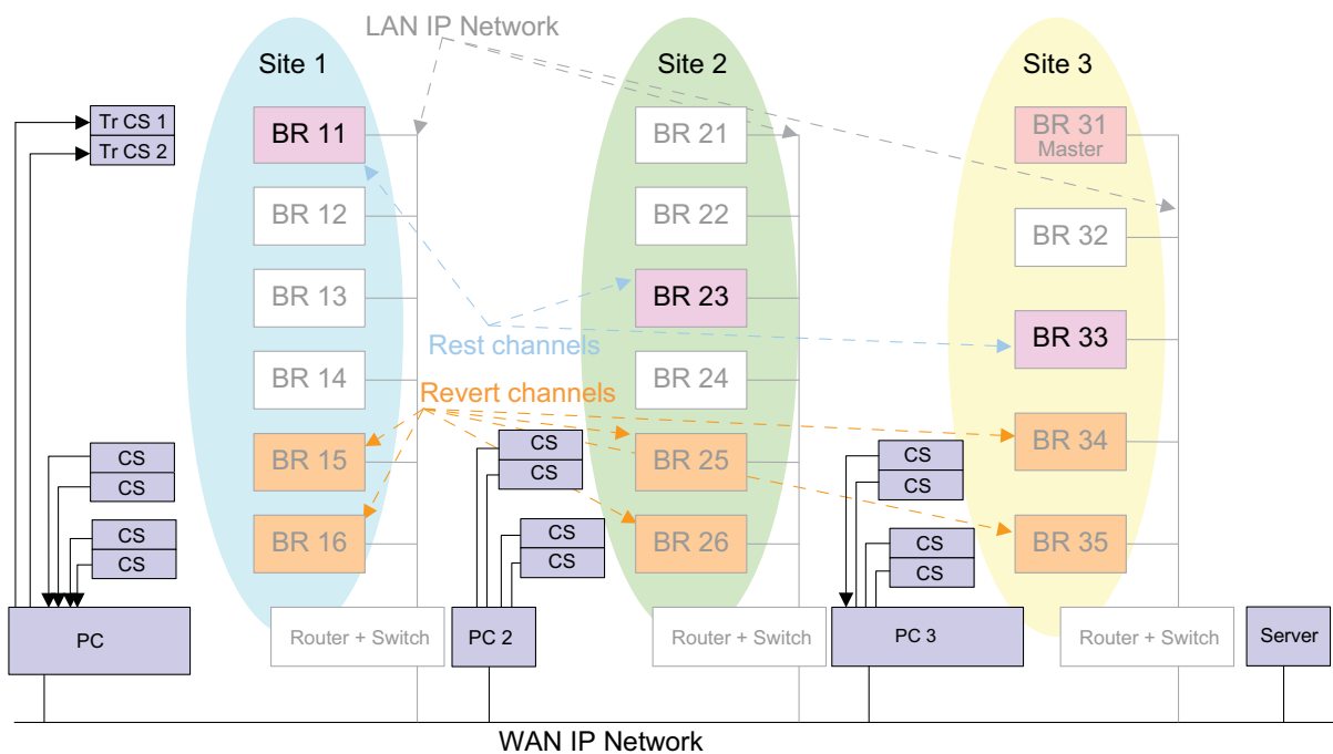
Figure 3-47 A Linked Capacity Plus System with Data over Local Revert Channels
