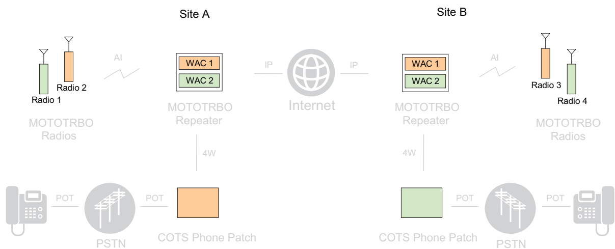
Figure 2-23 Two APP Boxes Supporting Two Wide Area Channels in IP Site Connect
