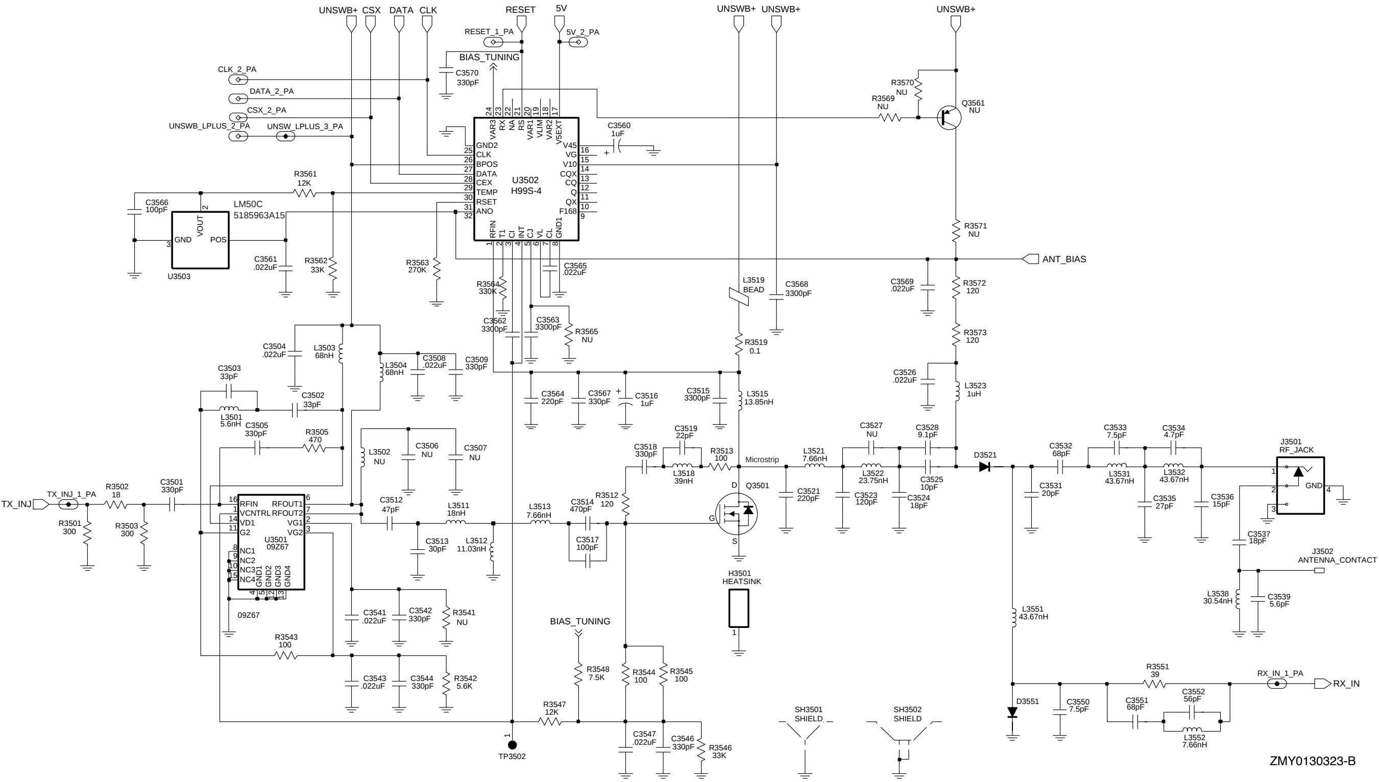
VHF (136-174 MHz) Transmitter Schematic Diagram
