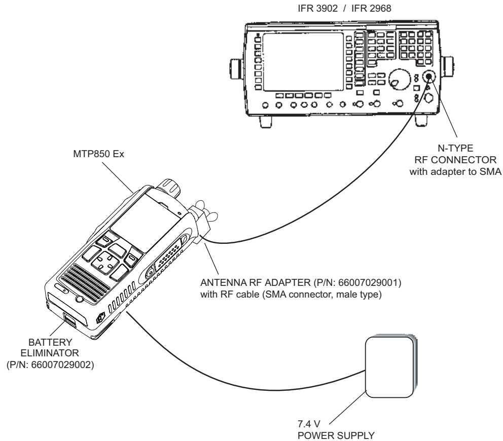
Figure 17 Typical Test Setup
