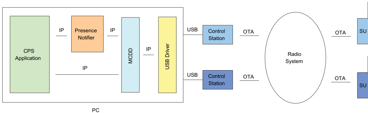
Figure 2-25 Multi-Channel Non-Remote CPS Application Configuration
