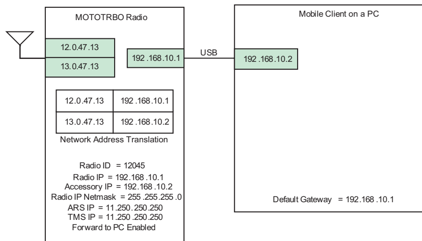
Figure 4-24 Air Interface Network Connectivity
