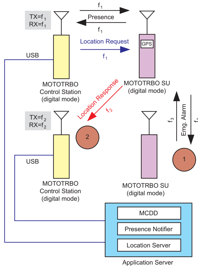
Figure 4-28 Emergency Alarm and GPS Revert Interaction Diagram
