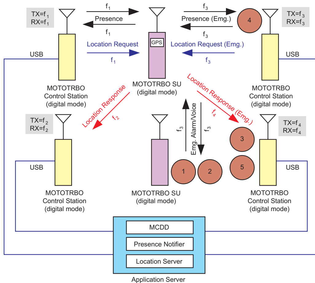
Figure 4-30 Emergency Alarm with Voice to Follow and GPS Revert Interaction Diagram
