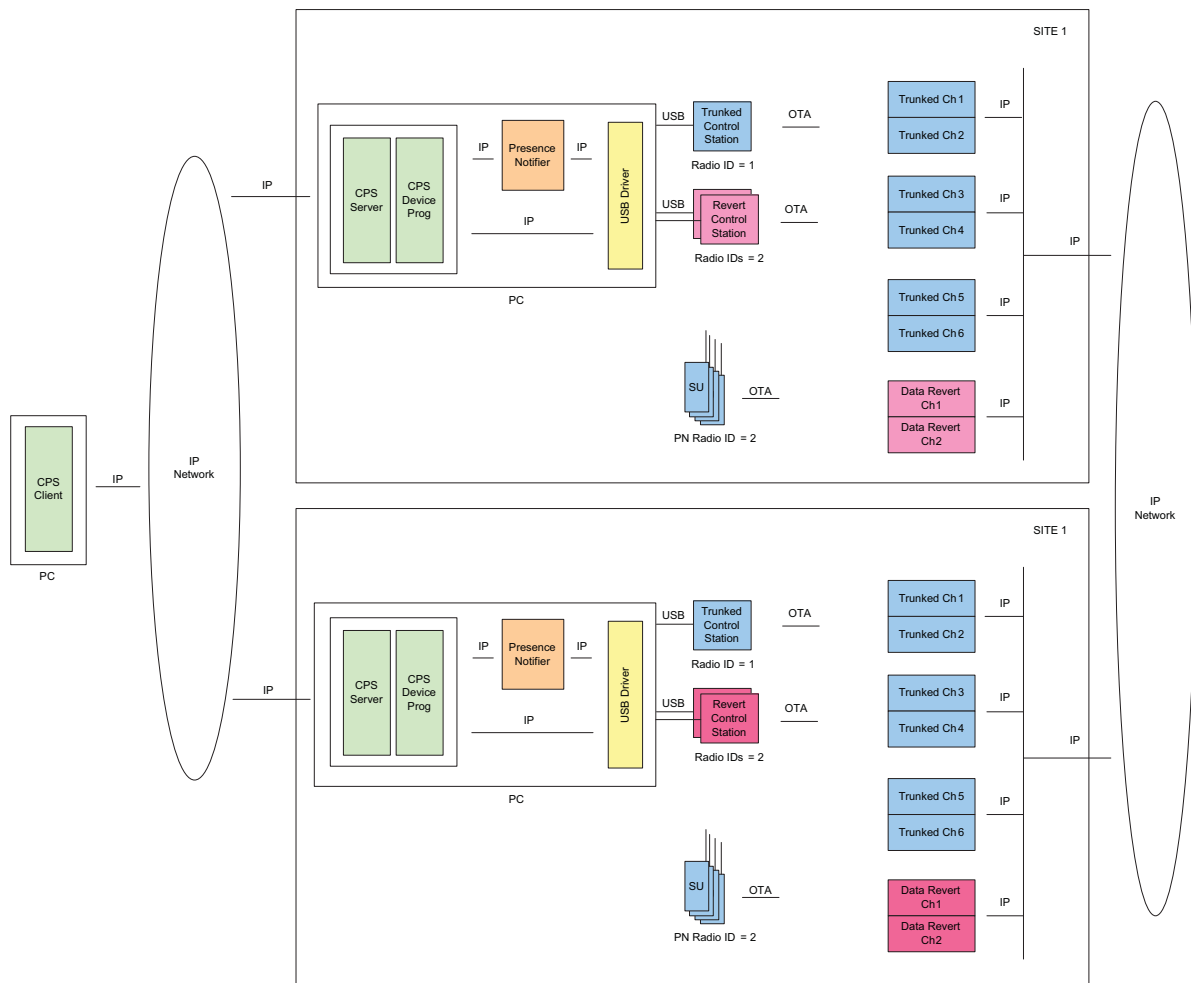
Figure 4-42 CPS Application in a Linked Capacity Plus System with a Presence Notifier and Local Area Data Revert Channels
