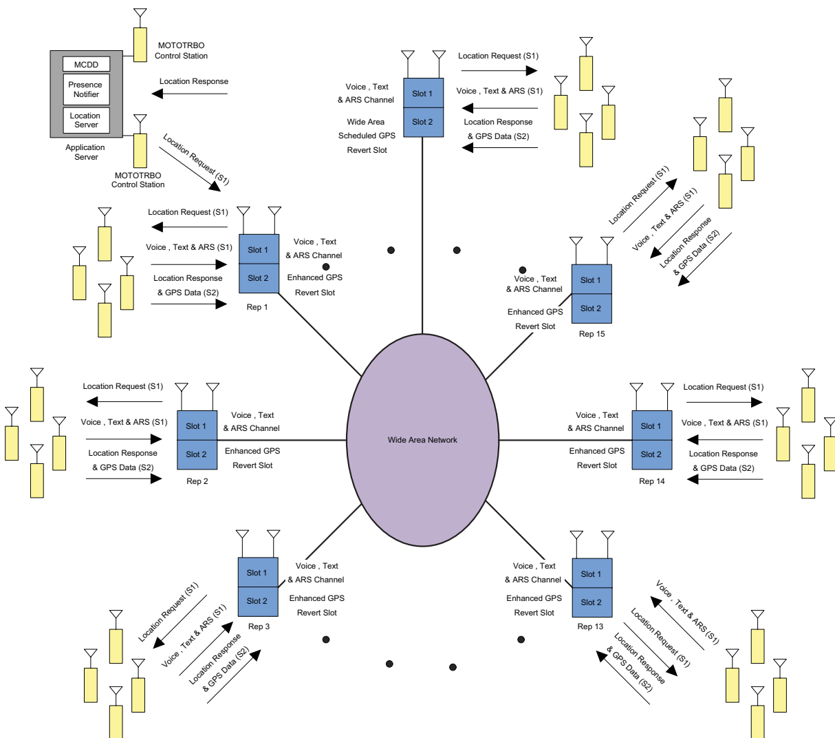
Figure 3-30 IP Site Connect System with an Enhanced GPS Revert Channel
