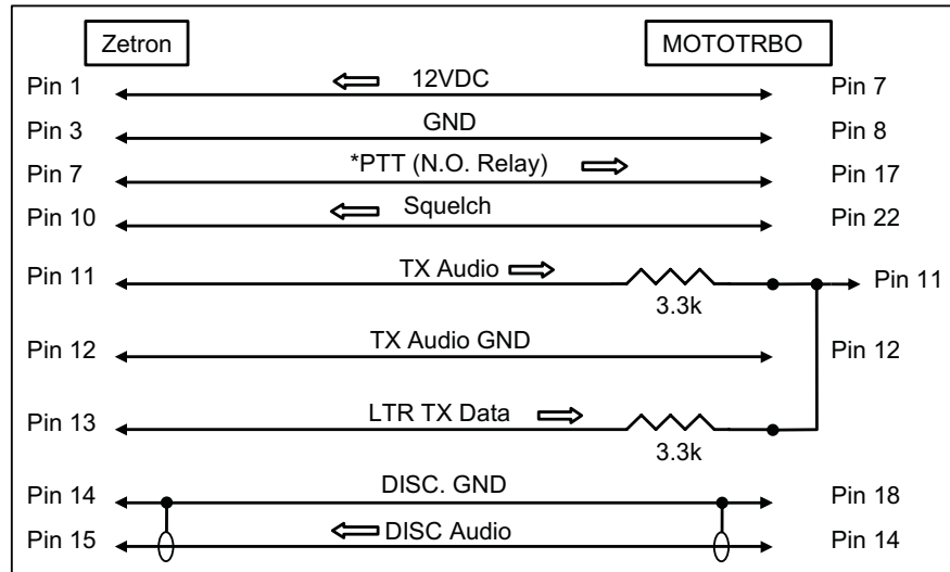
Figure 2-33 XPR 8300/XPR 8380/XPR 8400 Cable Schematic for Zetron Controllers
