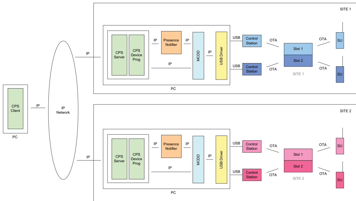
Figure 4-34 CPS Application Covering RF Isolated Single Site Repeaters
