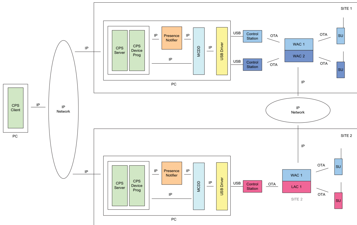
Figure 4-35 CPS Application in IP Site Connect Mode Covering Local Channels
