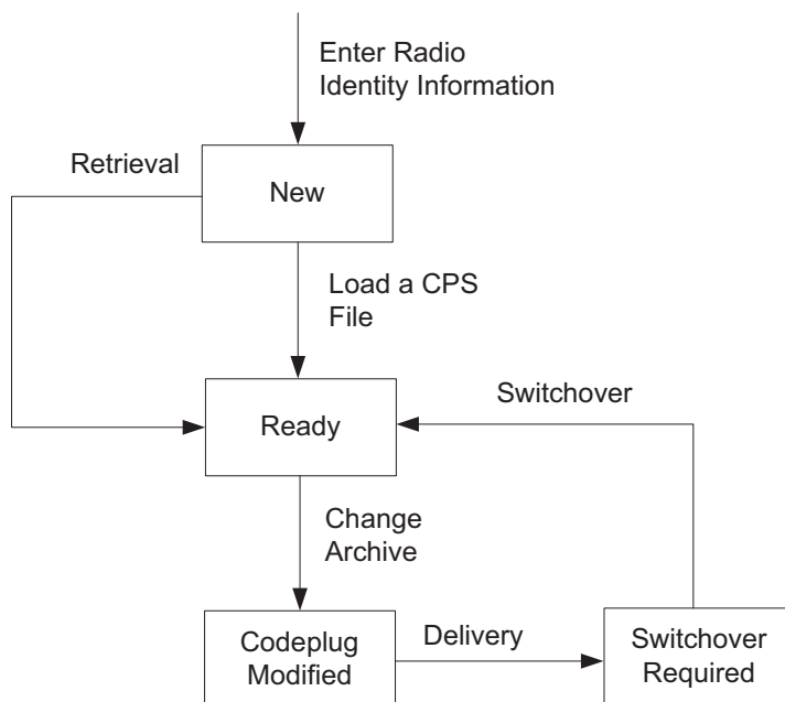
Figure 2-26 Over-the-Air Programming Process Flow Chart
