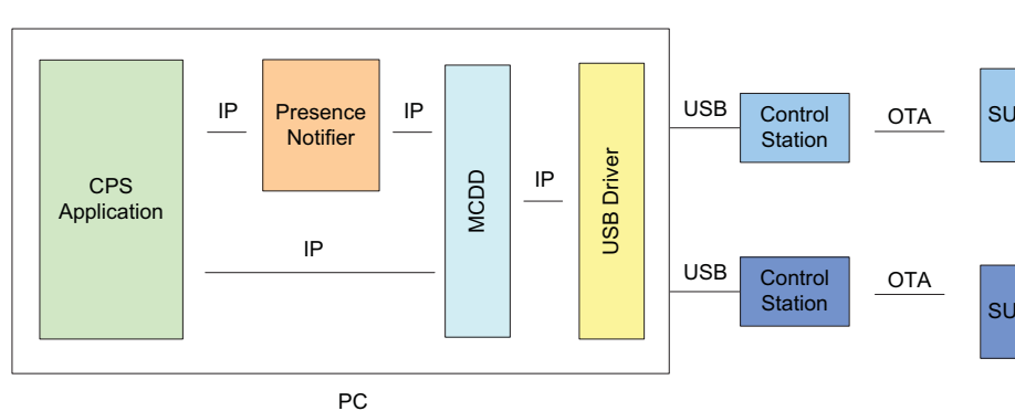
Figure 4-31 Multi-Channel CPS Application in Direct Mode
