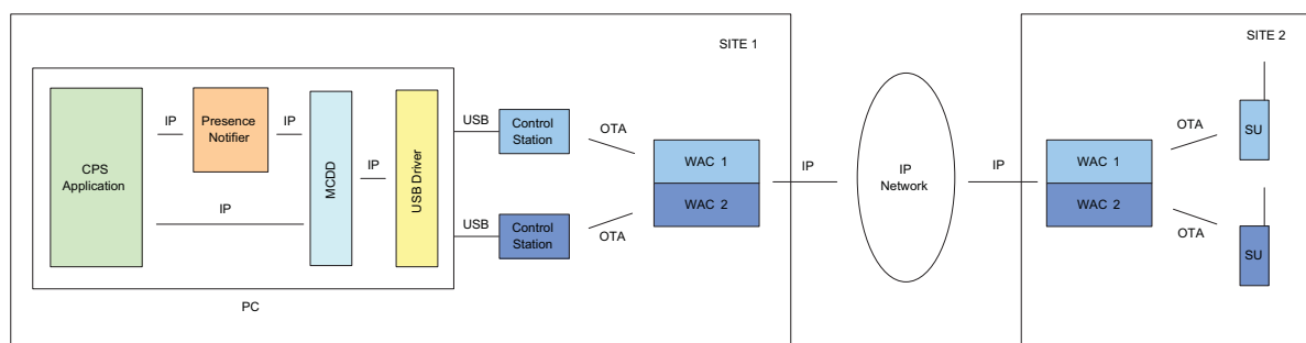
Figure 4-33 Multi-Channel CPS Application in IP Site Connect Mode
