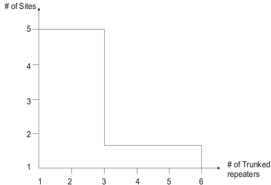
Figure 4-22 Valid Combinations of Sites and Trunked Repeaters for Linked Capacity Plus
