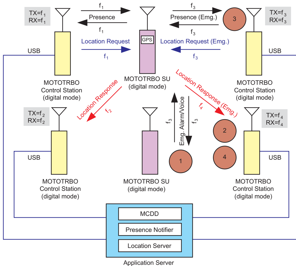
Figure 4-29 Emergency Alarm and Call and GPS Interaction Diagram
