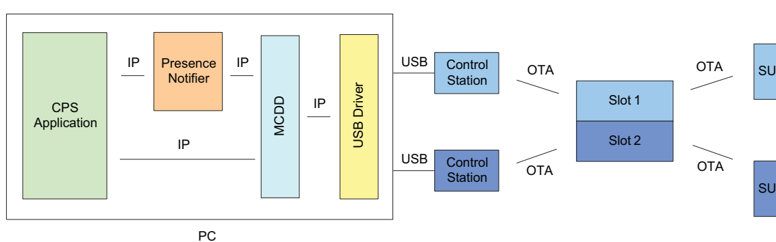
Figure 4-32 Multi-Channel CPS Application in Single Site Repeater Mode
