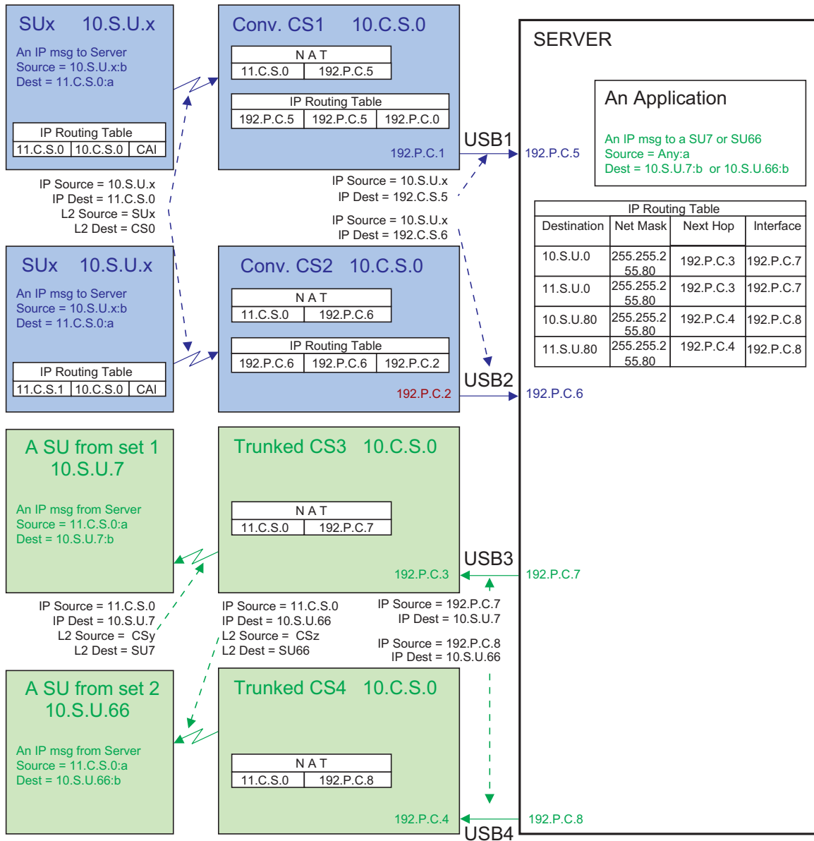
Figure 4-27 An example showing IPv4 addresses in a Capacity Plus configuration with Data Revert
