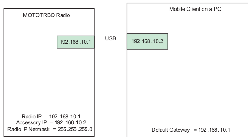
Figure 4-23 Connectivity between the Mobile Client and the MOTOTRBO Radio
