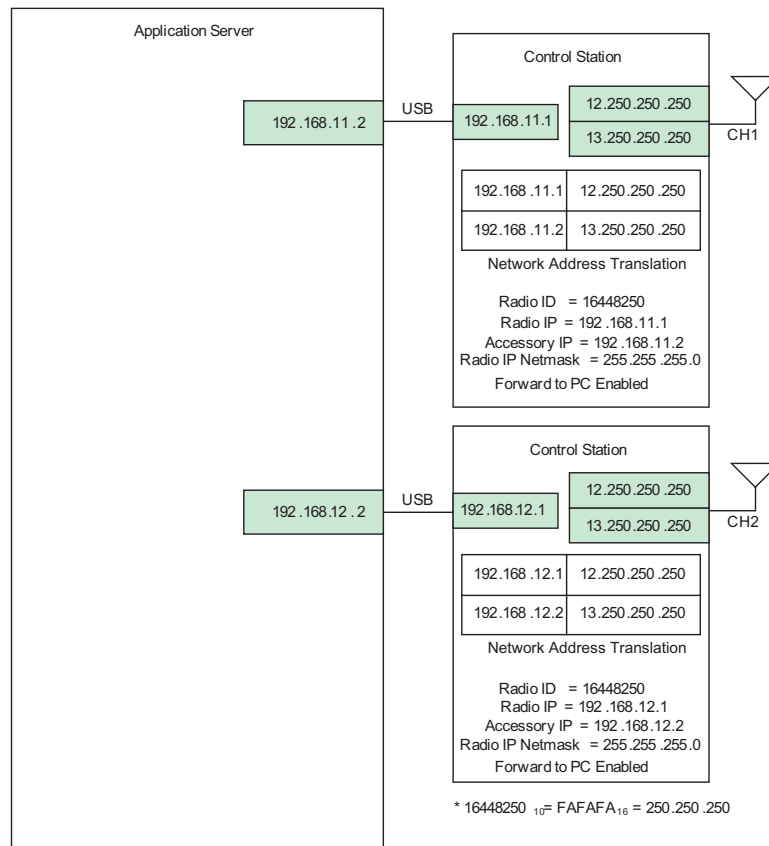
Figure 4-25 Application Server Control Station Network Connectivity
