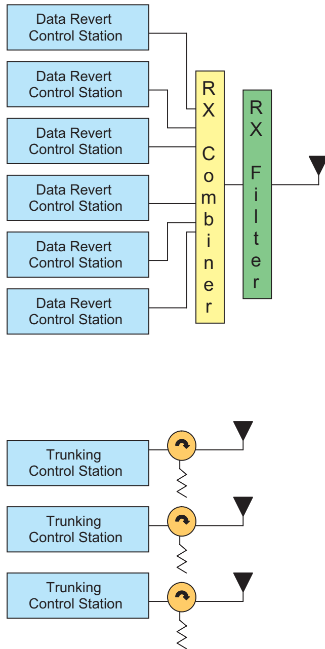
Figure B-1 Installation of Control Stations for Unconfirmed Data
