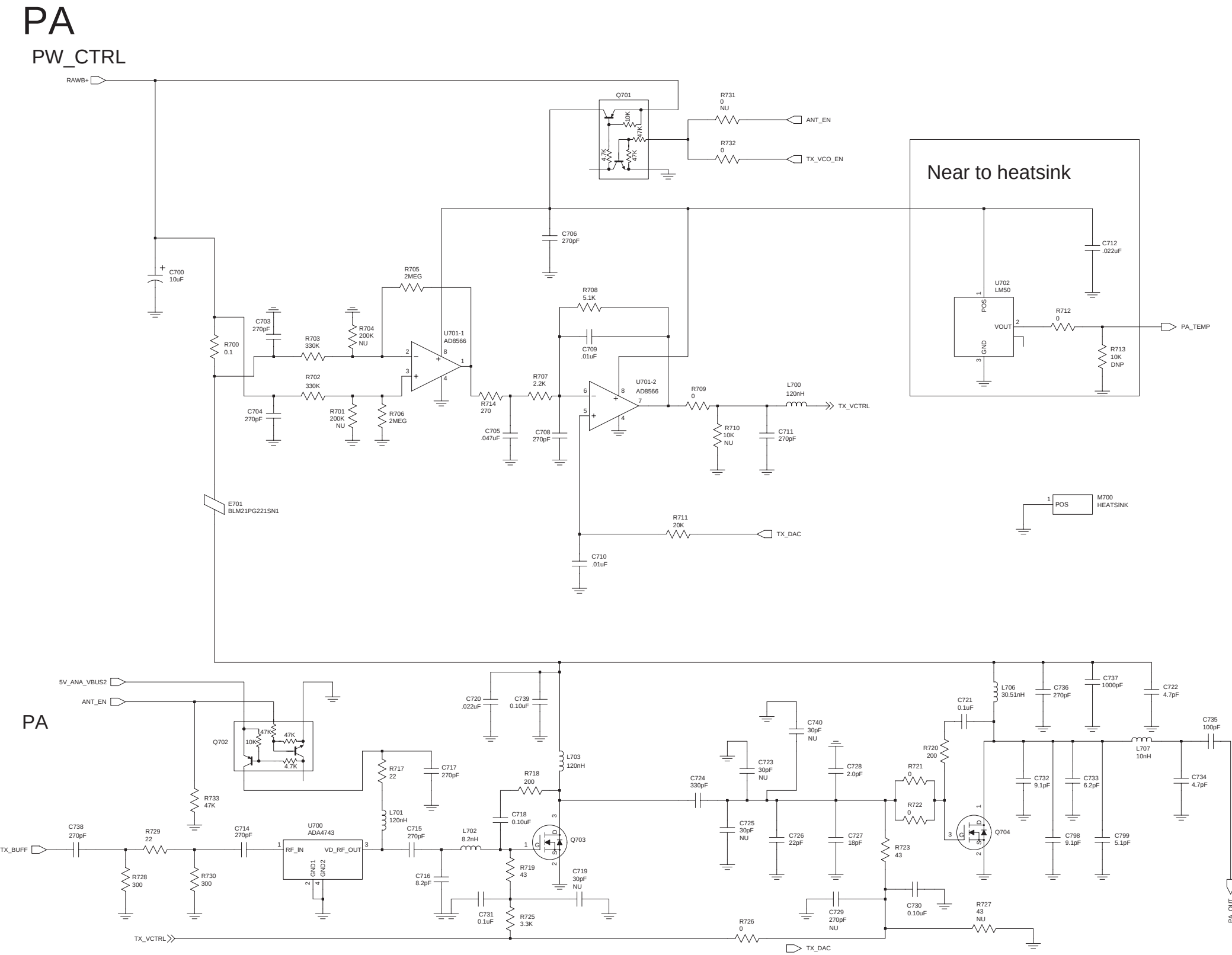
UHF2 Transmitter Schematic Diagram
