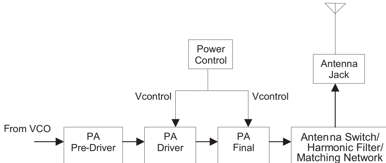
Figure 7-1: UHF Transmitter Block diagram
