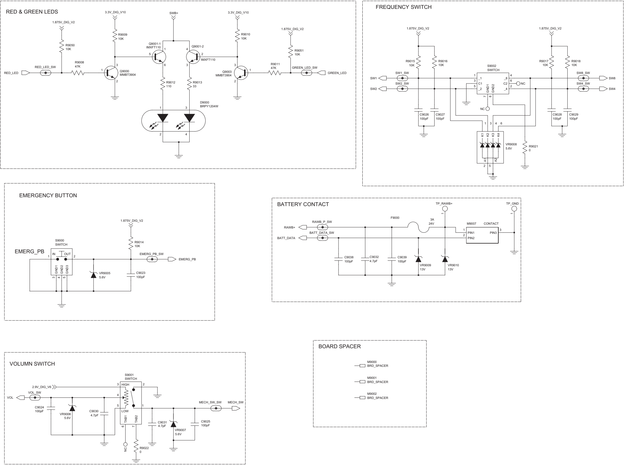
Controls and Switches Schematic Diagram (for 8486716Z16) *Emergency Button not applicable for XPR 6100*
