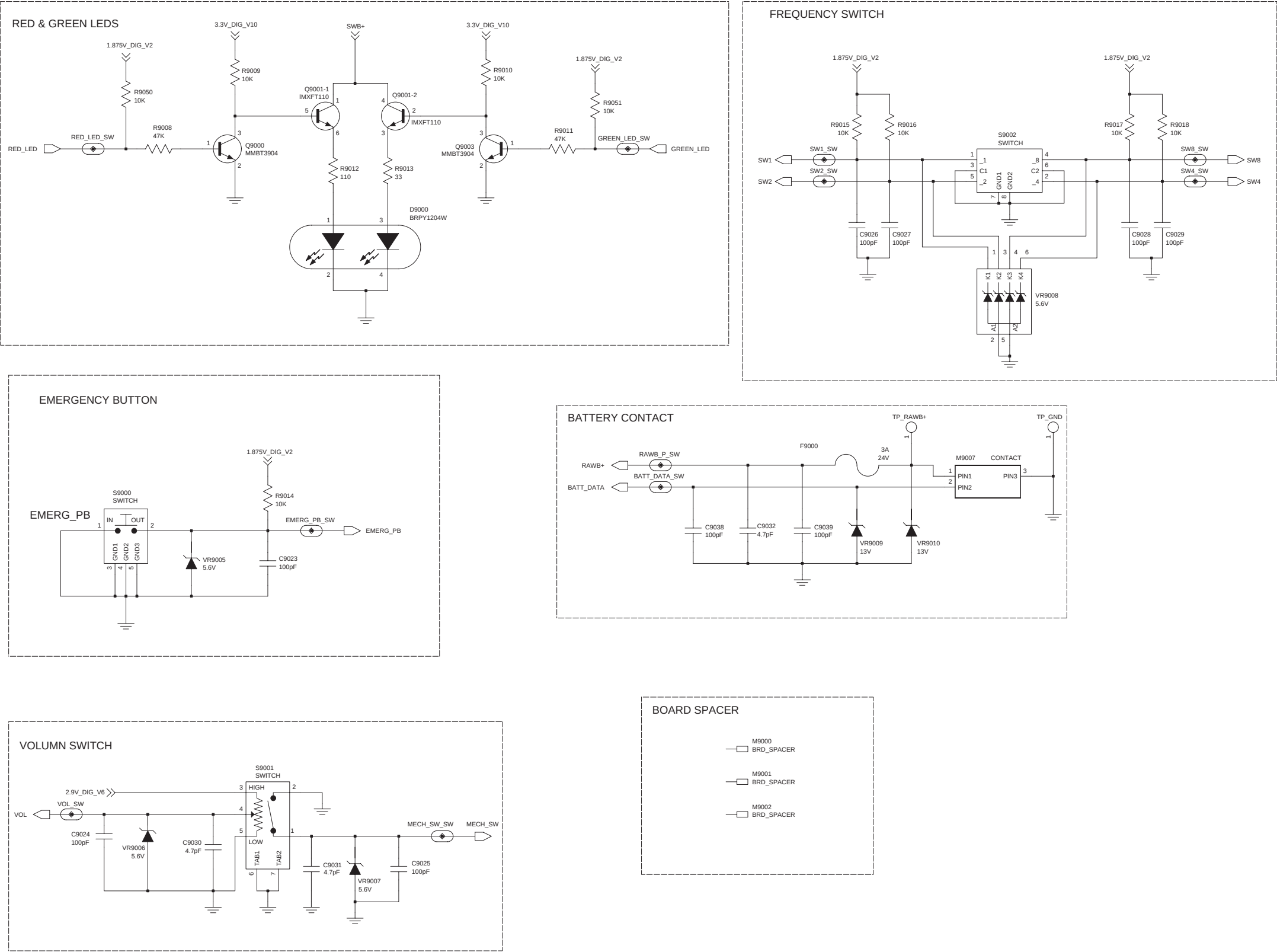
Controls and Switches Schematic Diagram (for 8486716Z07/8486716Z13, 8486716Z08 & 8475130M01) *Emergency Button not applicable for XPR 6100*
