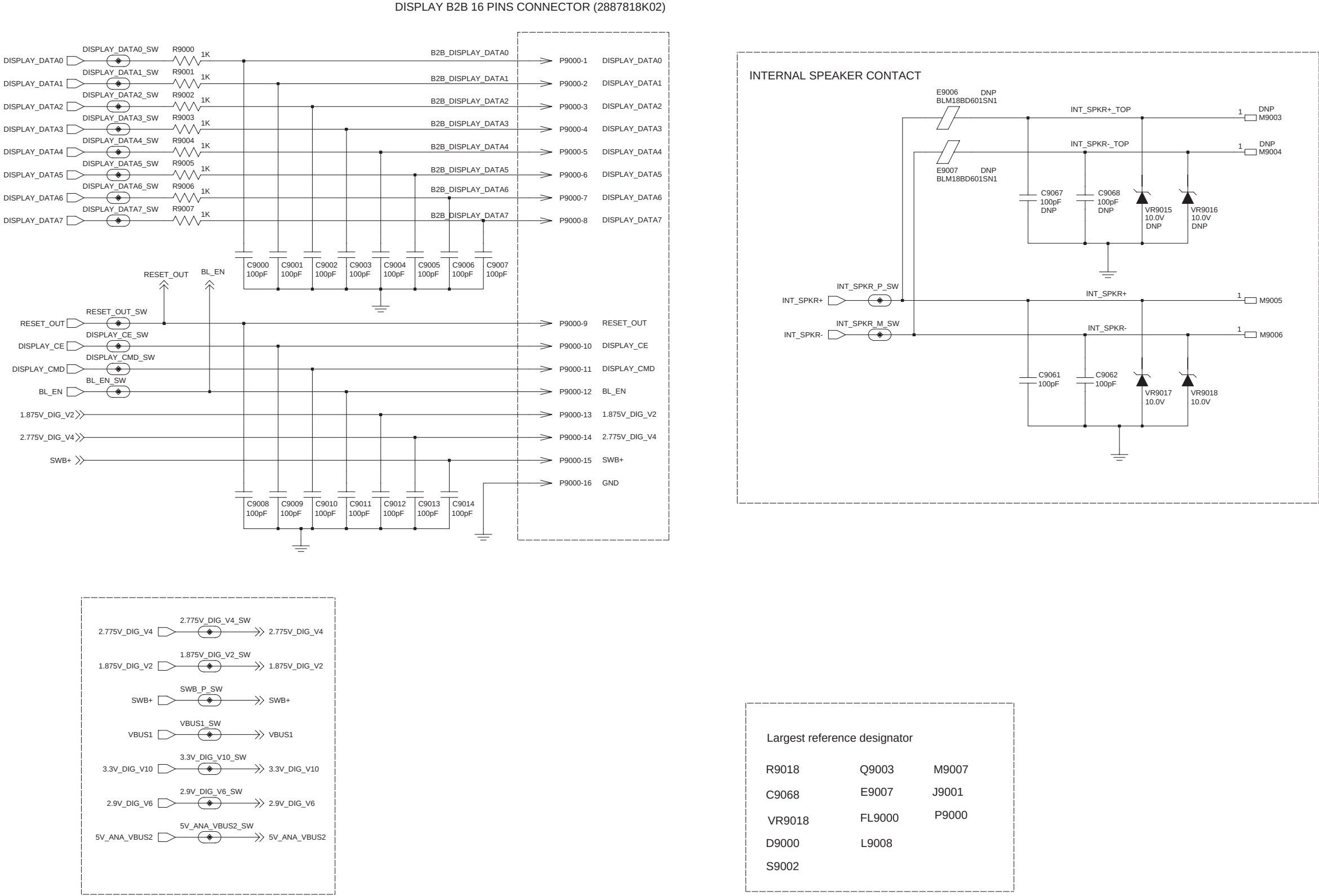
Controller LCD and Speaker Interface Schematic Diagram (for 8486716Z04, 8486716Z07/8486716Z13, 8486716Z08 & 8475130M01)
