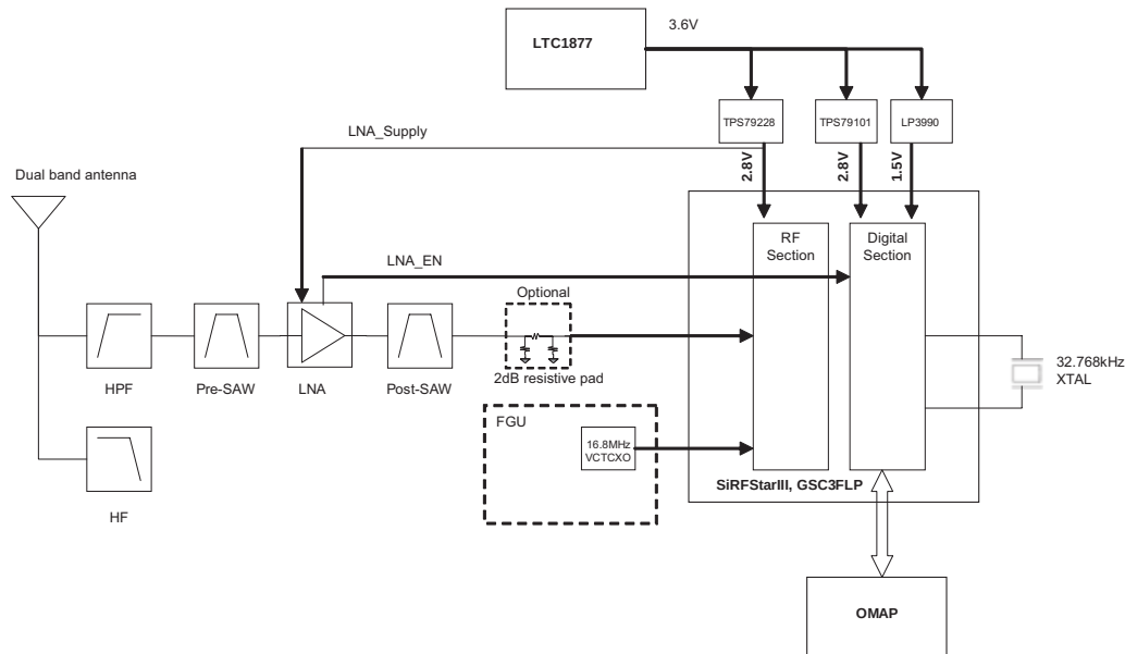
Figure 6-5: GPS Receiver Block Diagram
