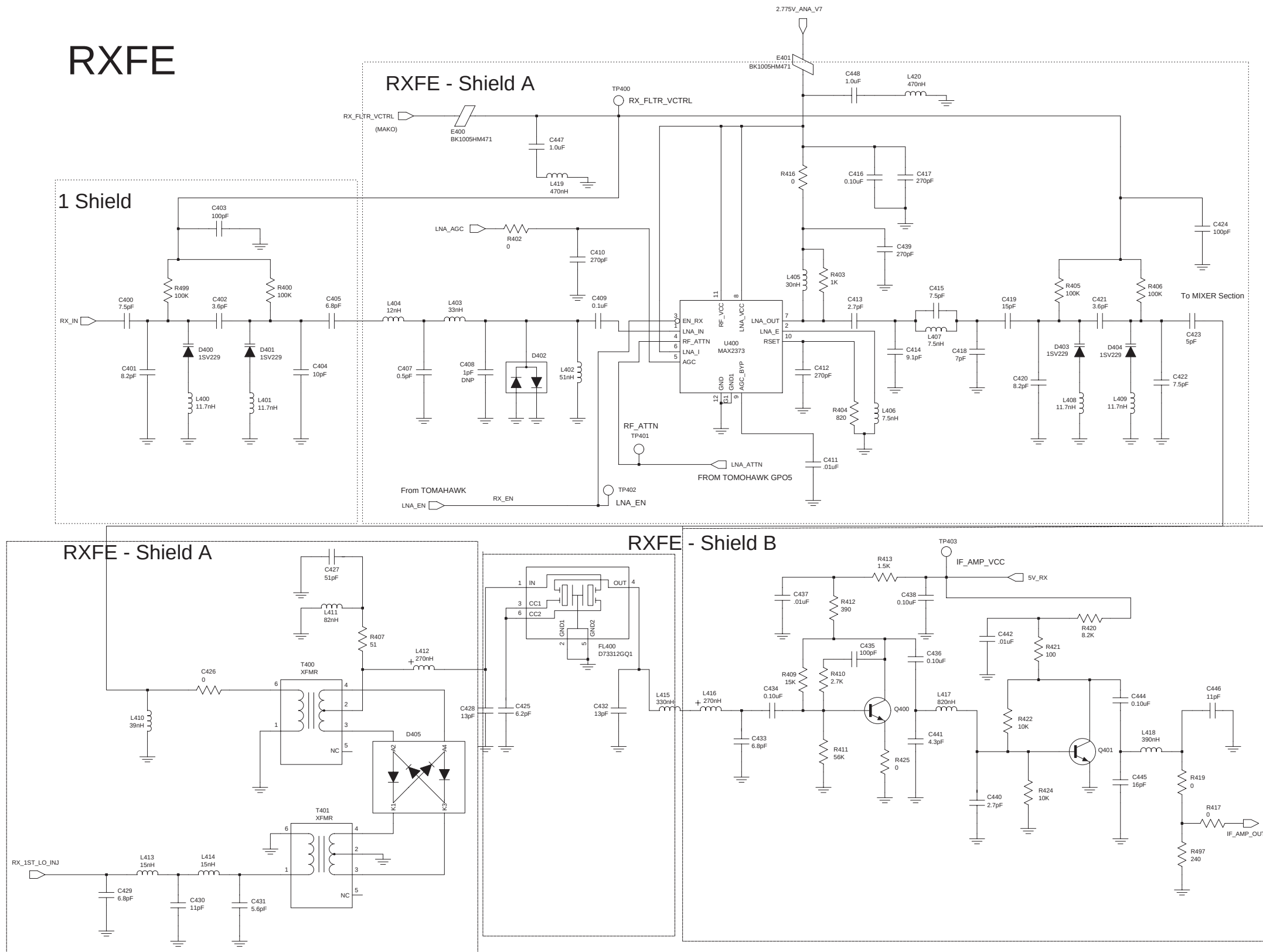
UHF2 Receiver Front End Schematic Diagram
