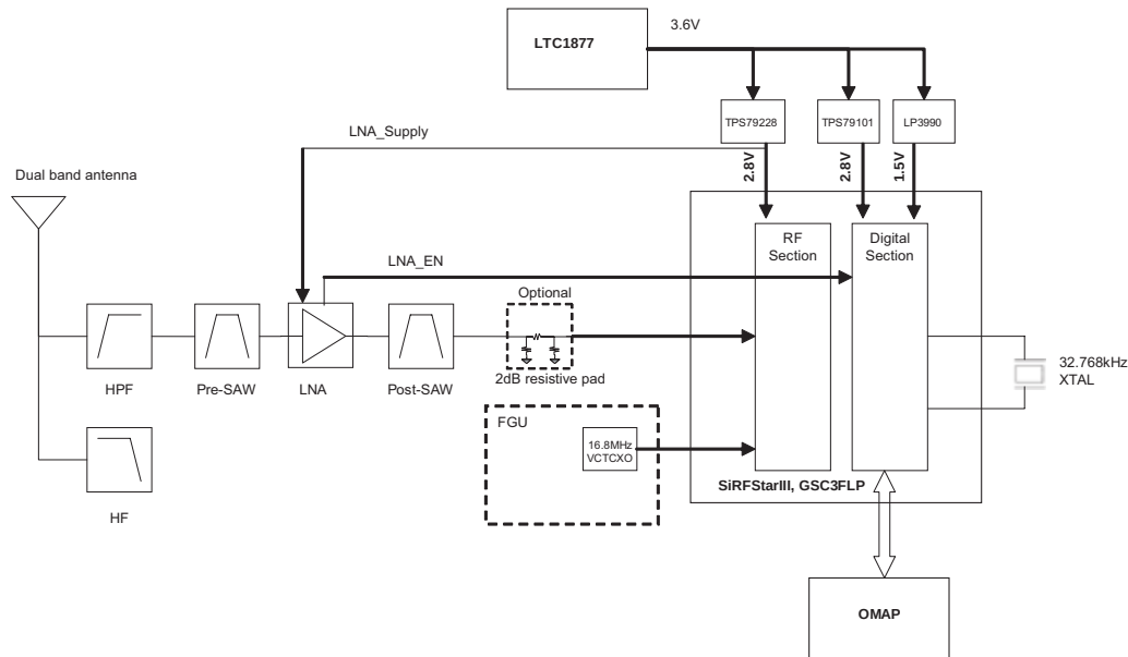
Figure 9-5: GPS Receiver Block Diagram
