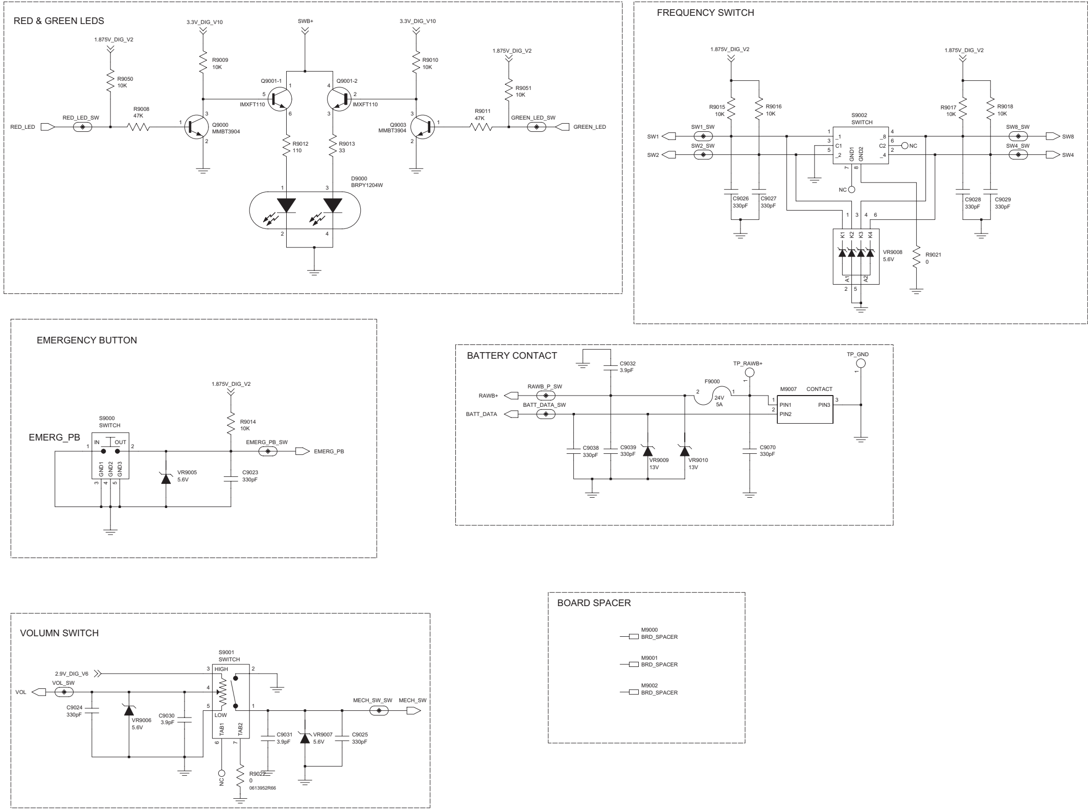
Controls and Switches Schematic Diagram (for 8415113H13) *Emergency Button not applicable for XPR 6100
