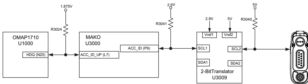
Figure 5-6: ACC_ID Interface Connections
