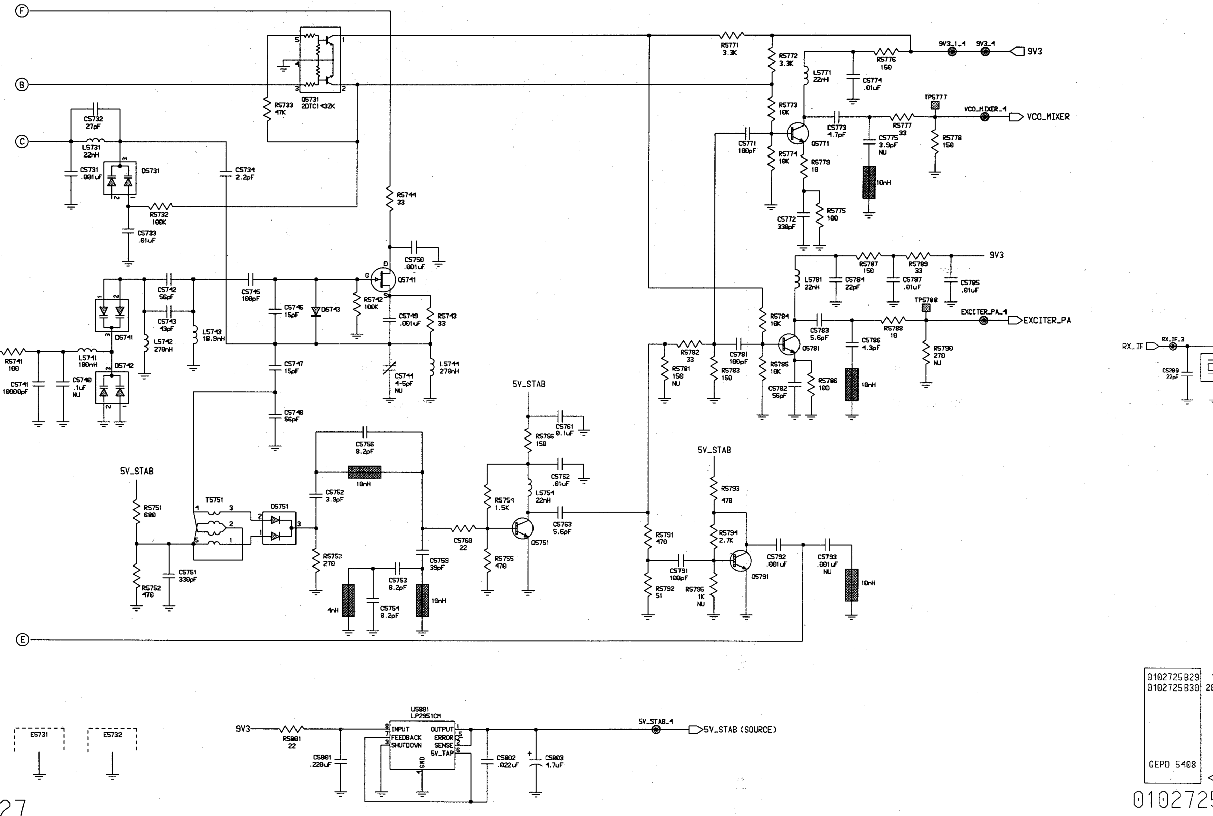
UHF Voltage Controlled Oscillator Schematic Diagram
