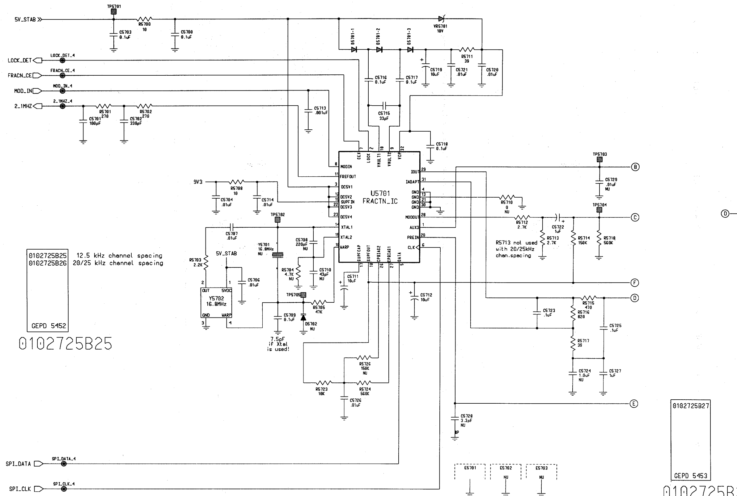
UHF Synthesizer Schematic Diagram
