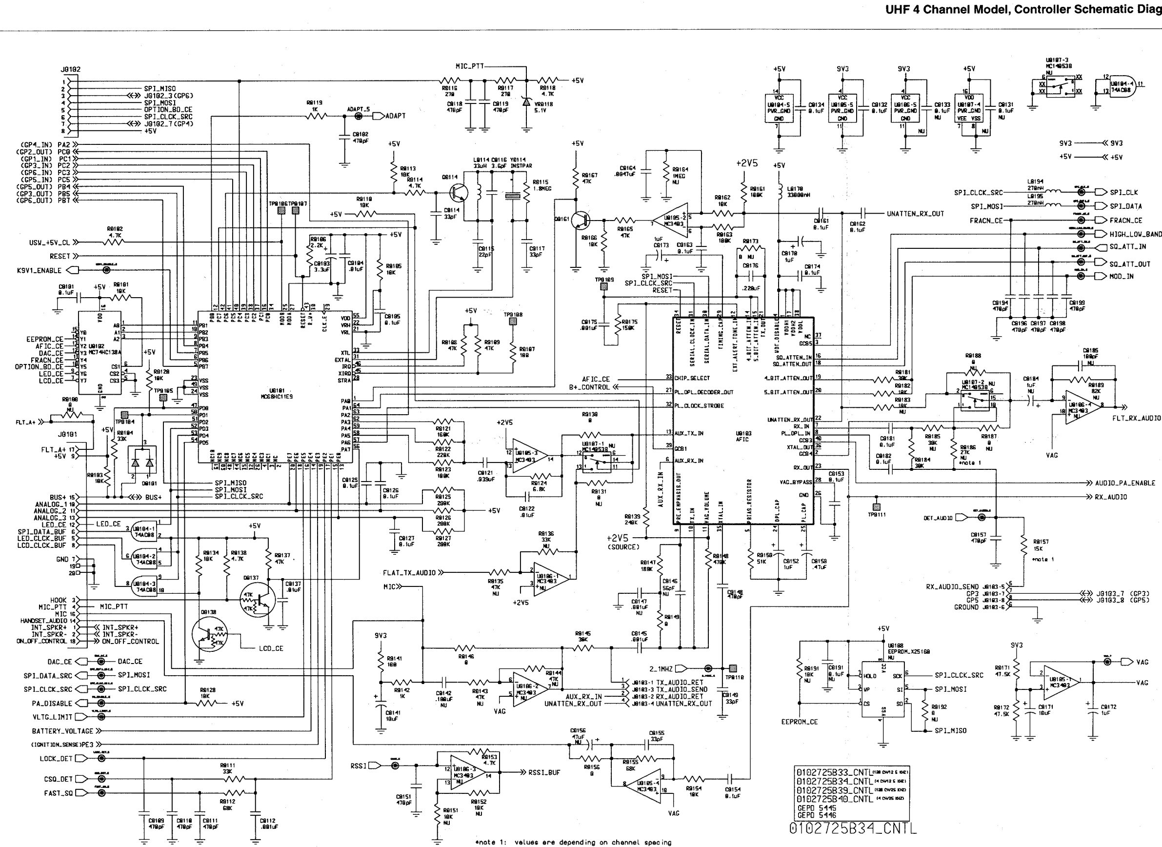
UHF 4 Channel Model, Controller Schematic Diagram 1 of 2
