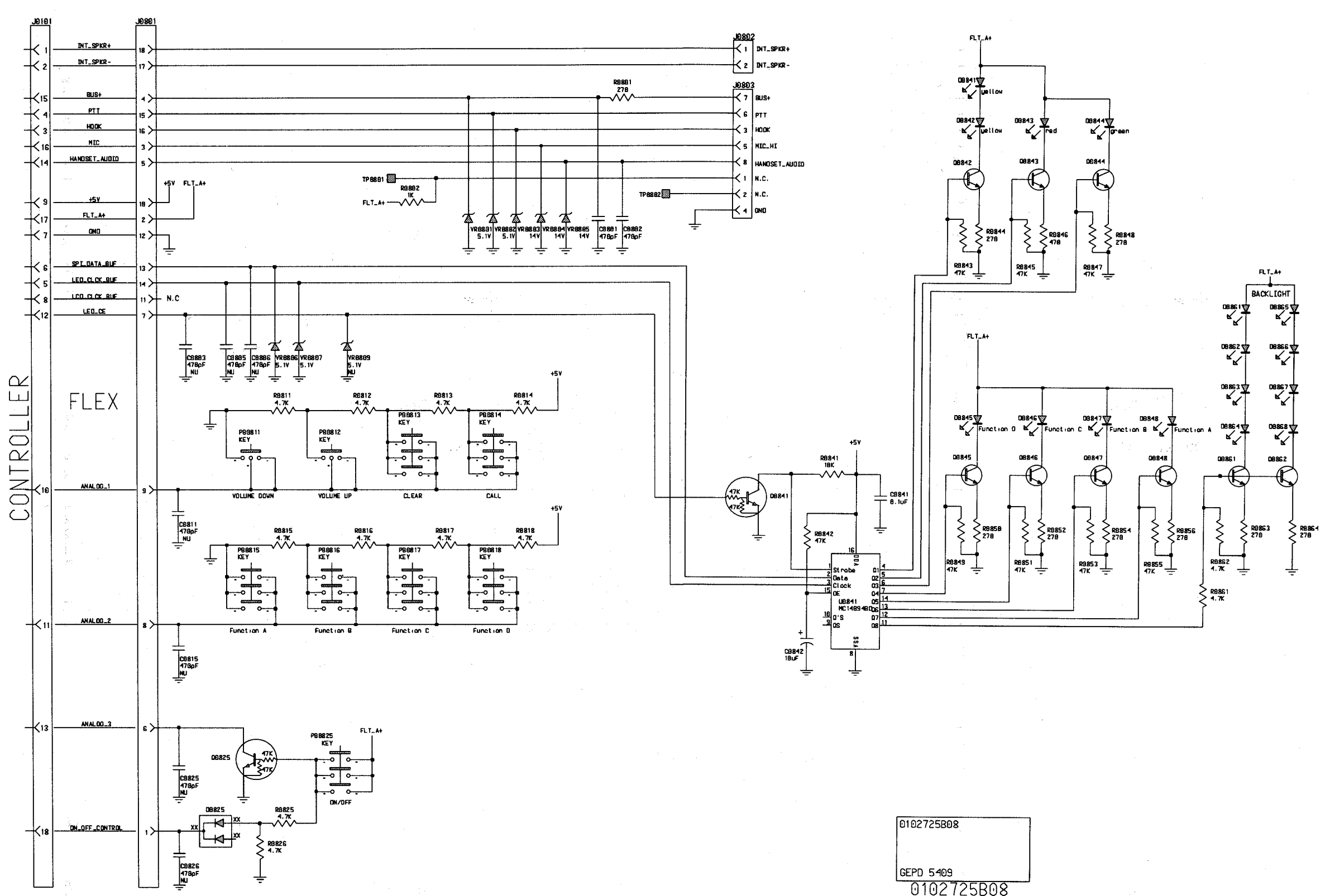
Control Head K Schematic Diagram
