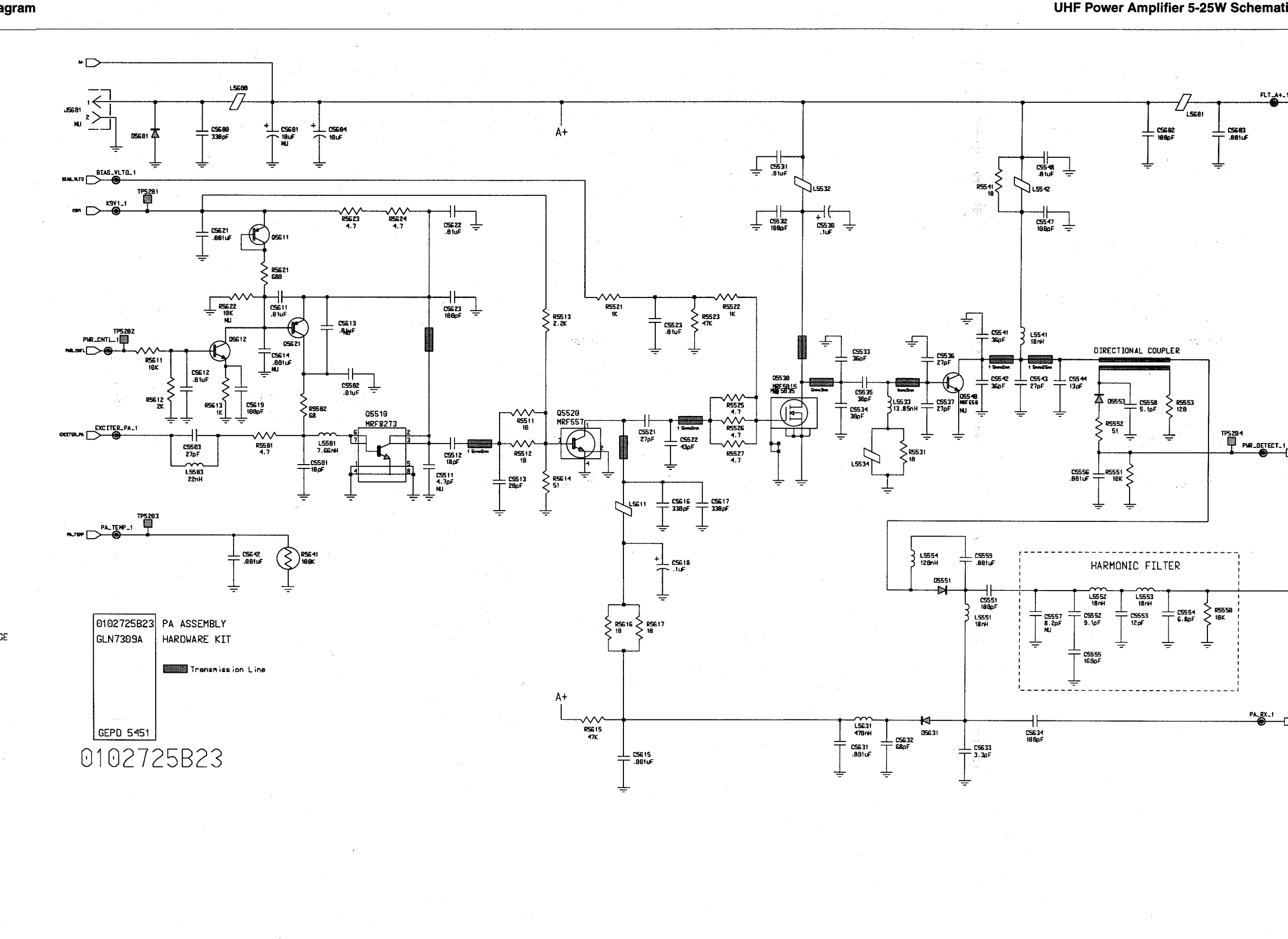
UHF Power Amplifier 5-25W Schematic Diagram
