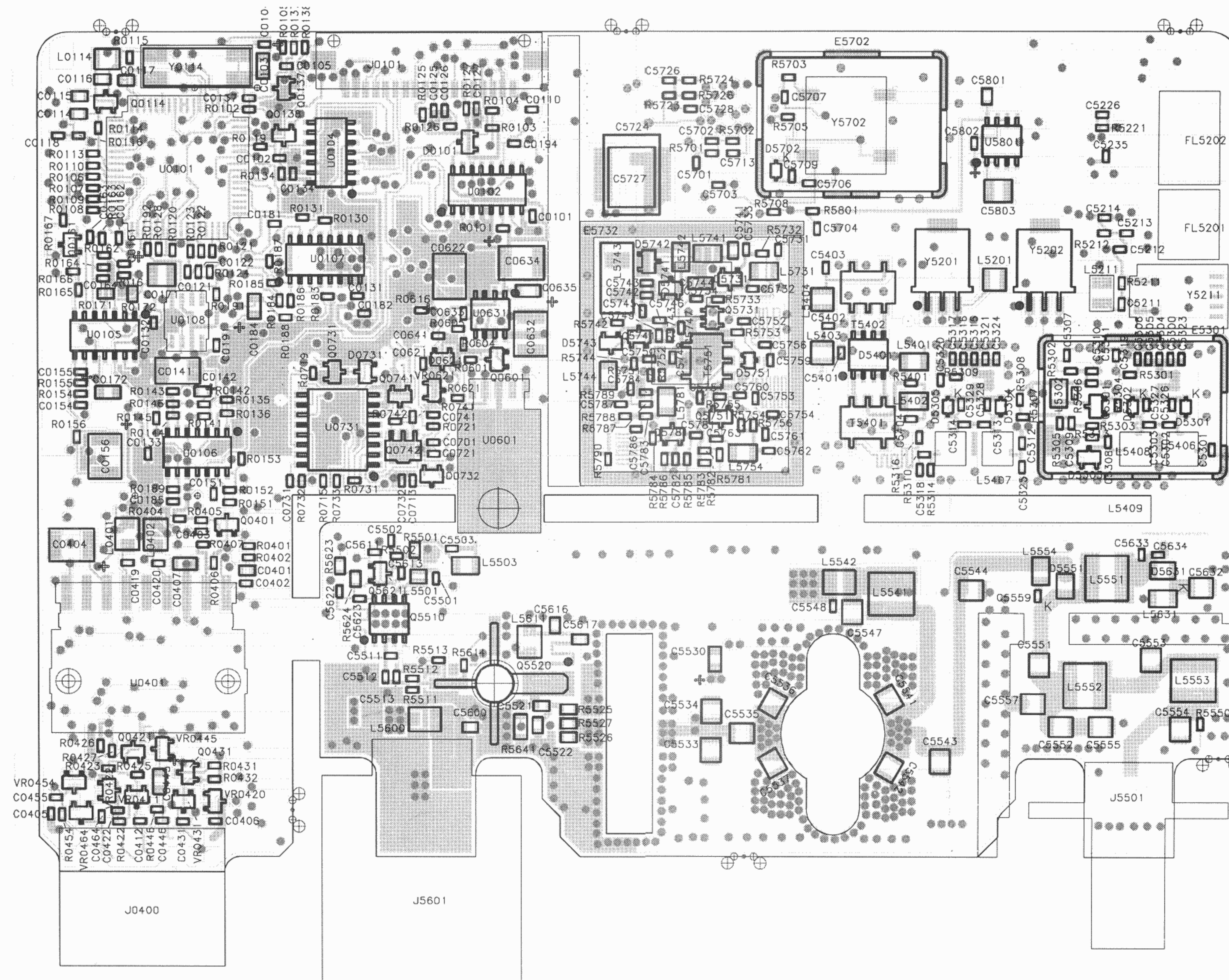
UHF Main Board Component Side PCB No. 8402624Y04
