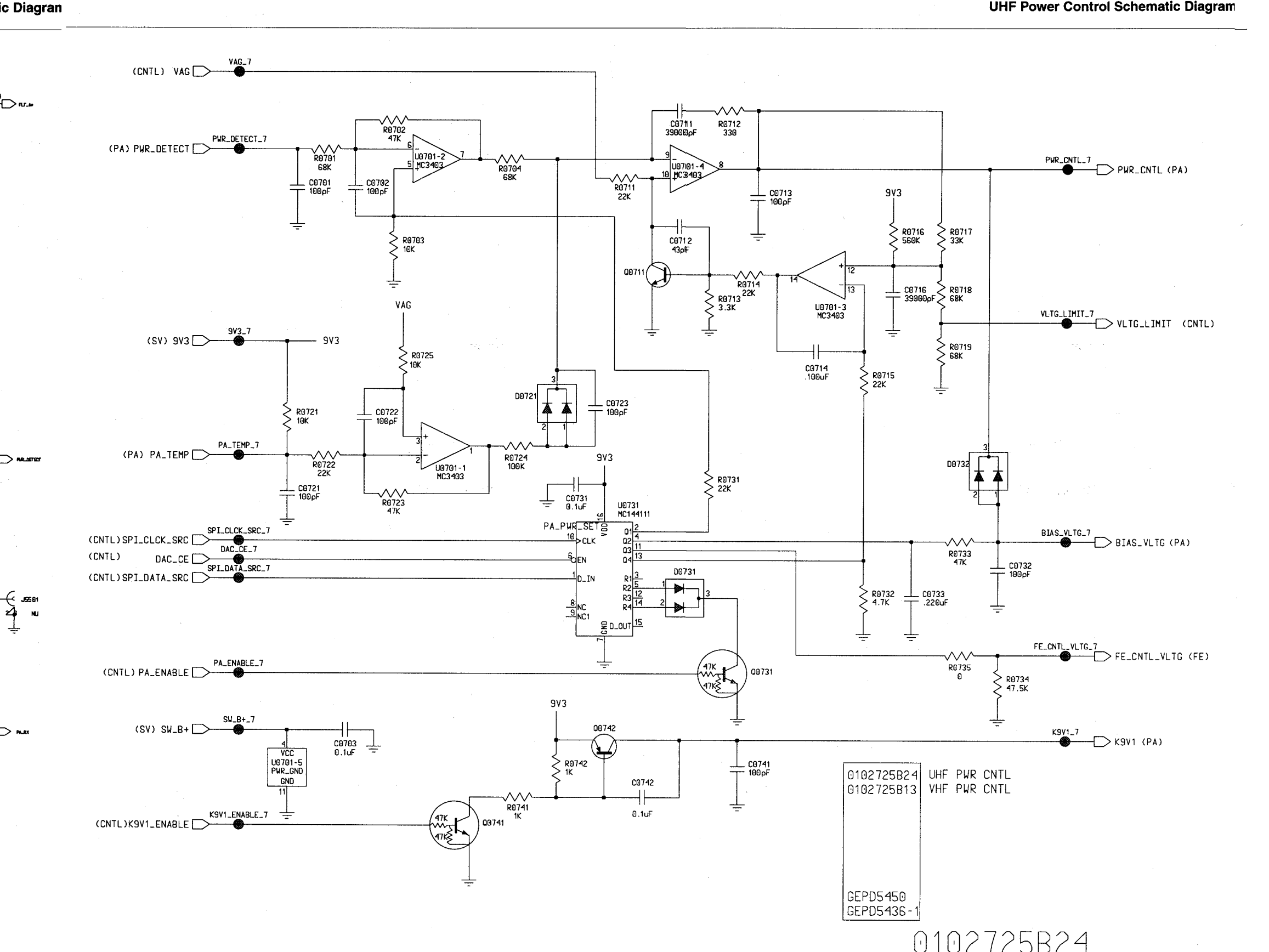
UHF Power Control Schematic Diagram
