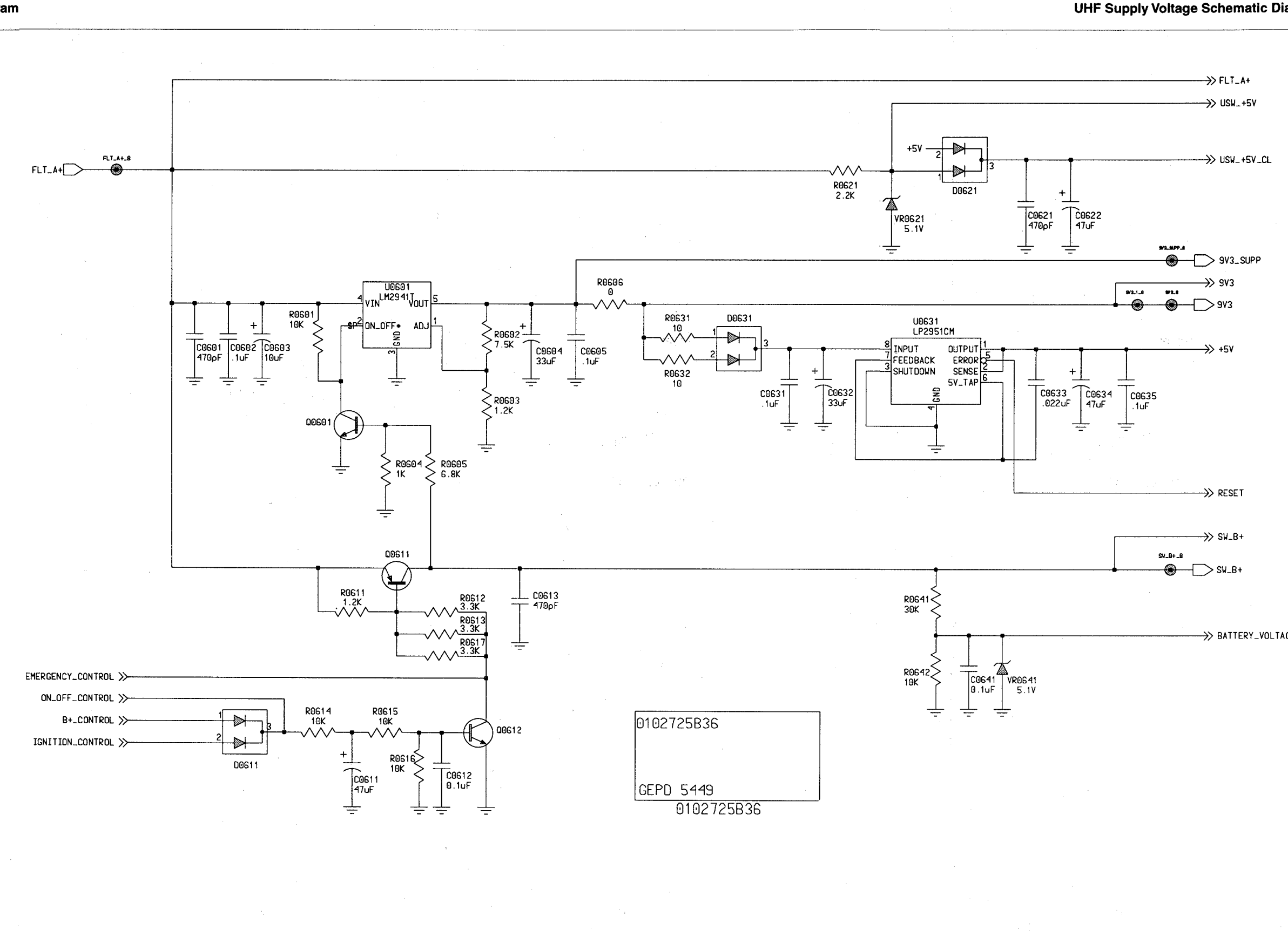
UHF Supply Voltage Schematic Diagram
