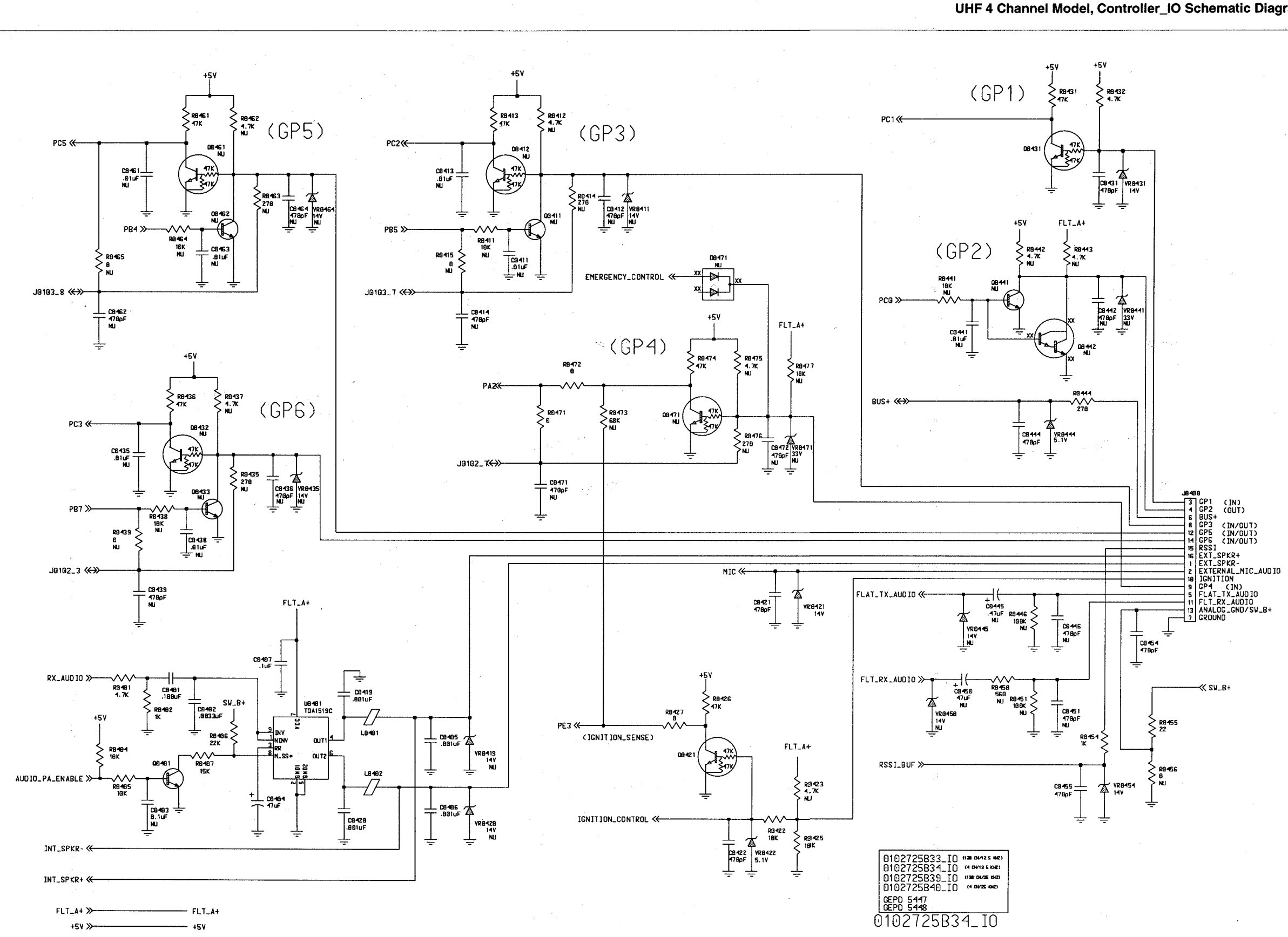
UHF 4 Channel Model, Controller_IO Schematic Diagram 2 of 2
