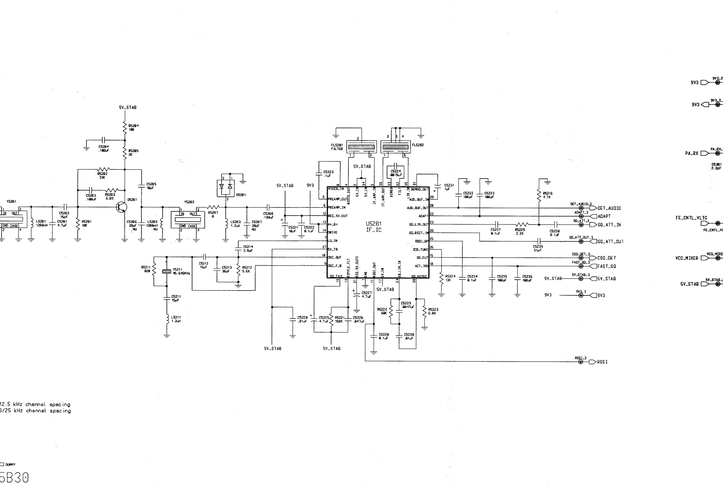
UHF RX-IF Schematic Diagram
