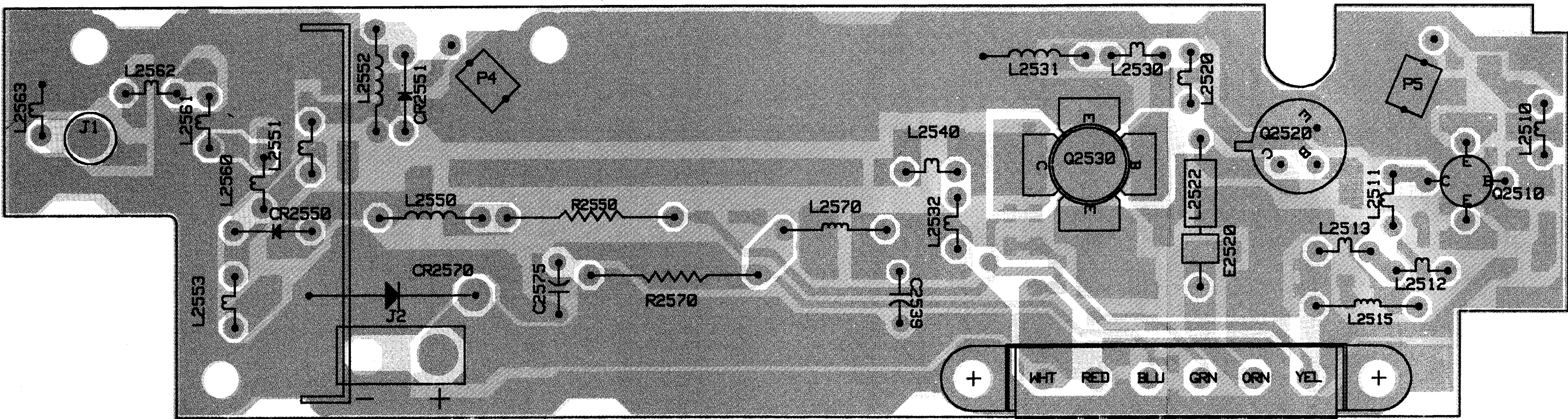
COMPONENT SIDE
