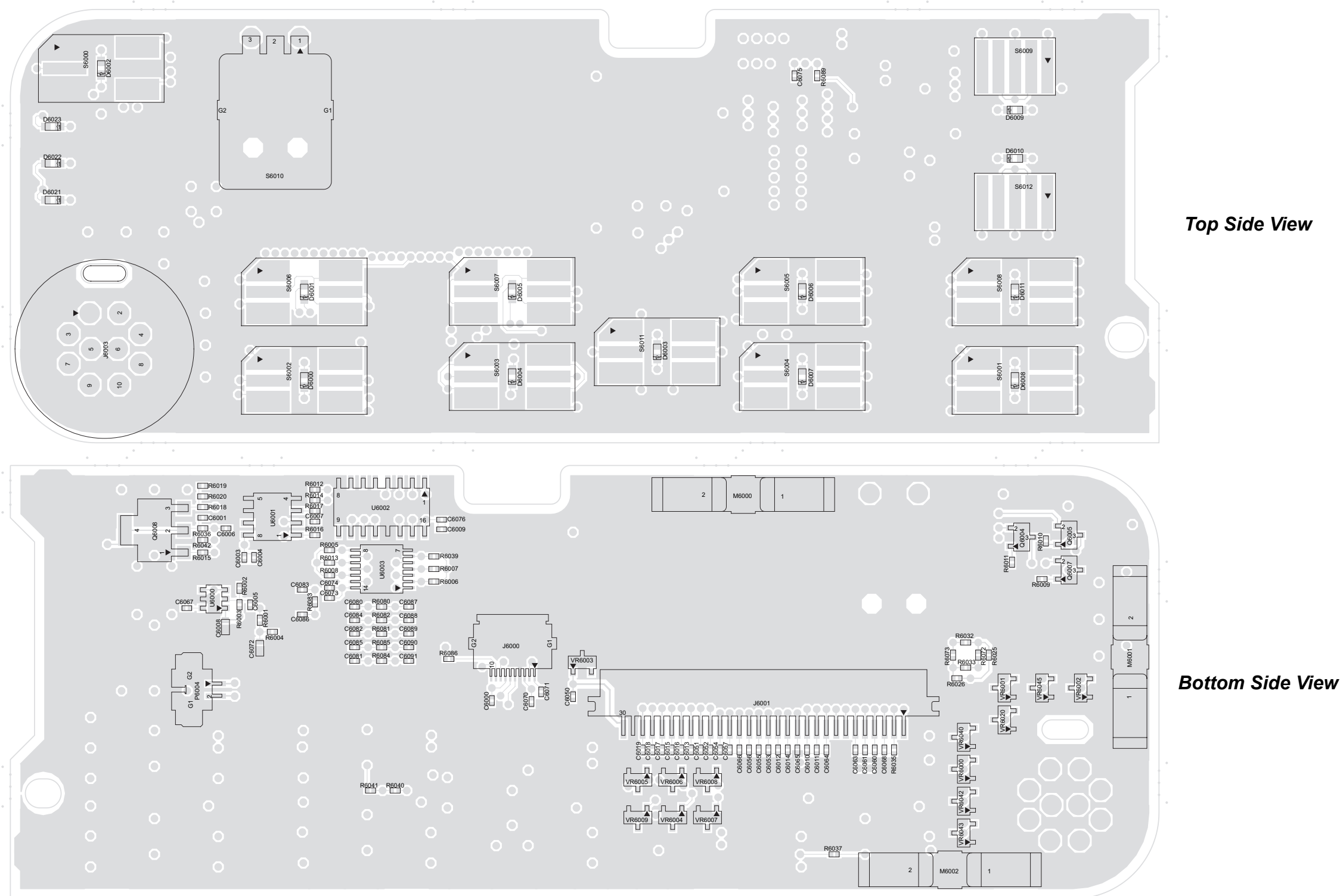
Display Control Head - PCB 8415026C08
