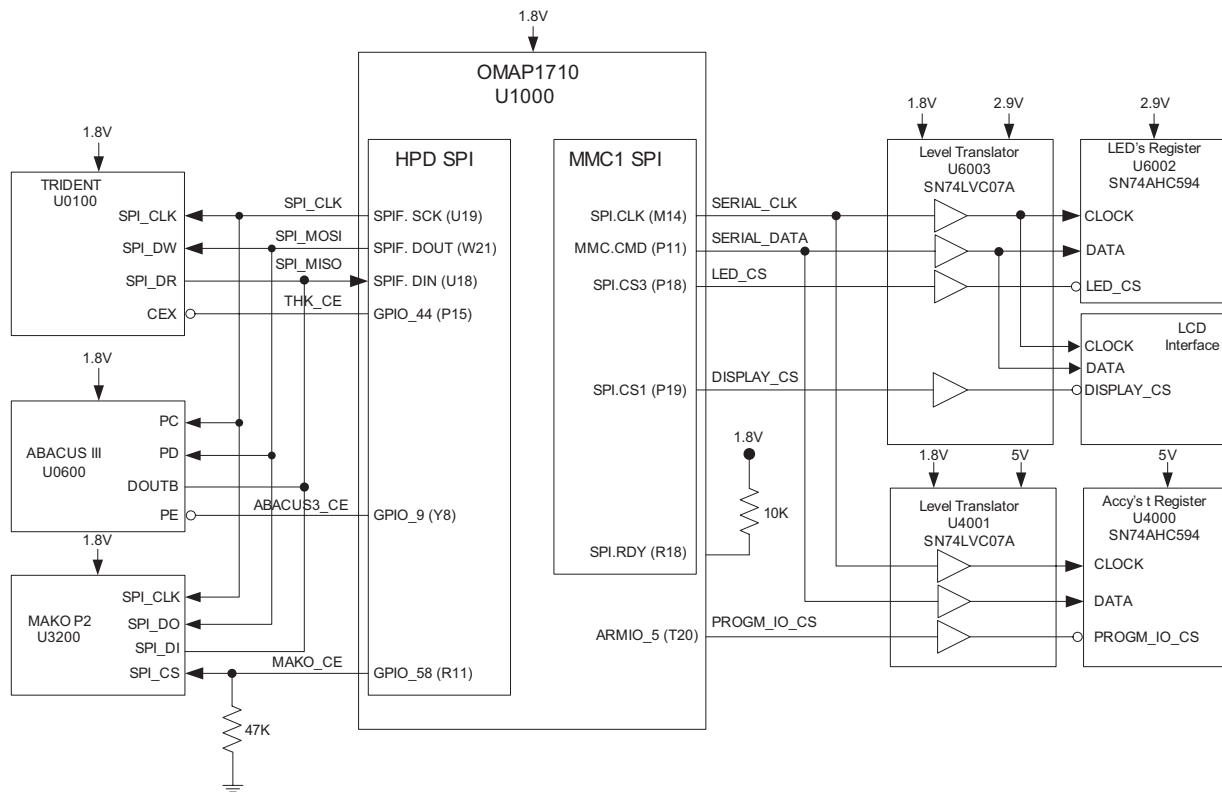
Figure 1-6 SPI Connections
