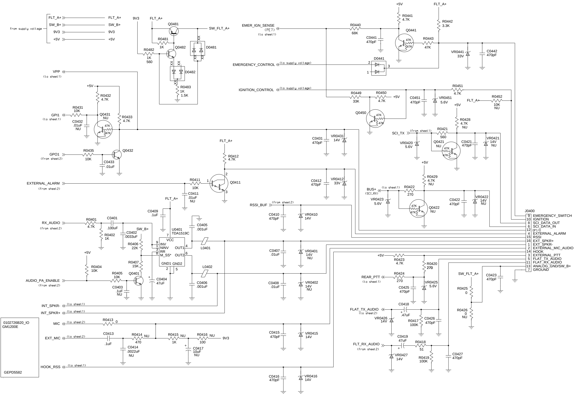
Controller_IO Schematic Diagram 3 of 3
