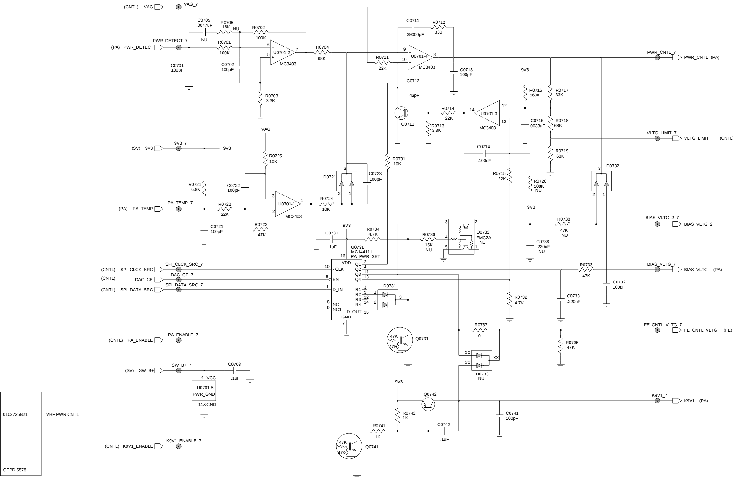
VHF (136-174MHz) Power Control Schematic Diagram
