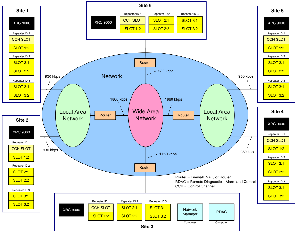
Figure 4-7 Example for Calculating Bandwidth Requirements w/o Secure VPN
