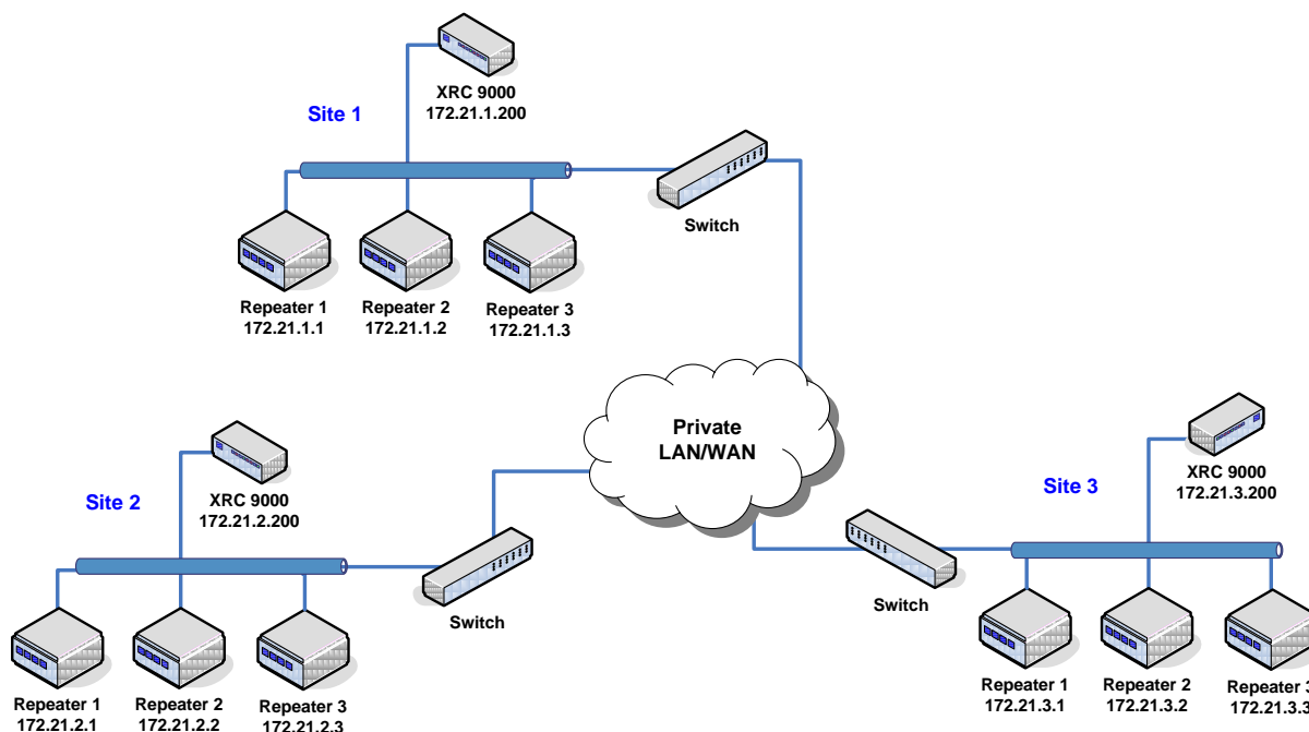
Figure 4-10 Simplified Example IP Plan
