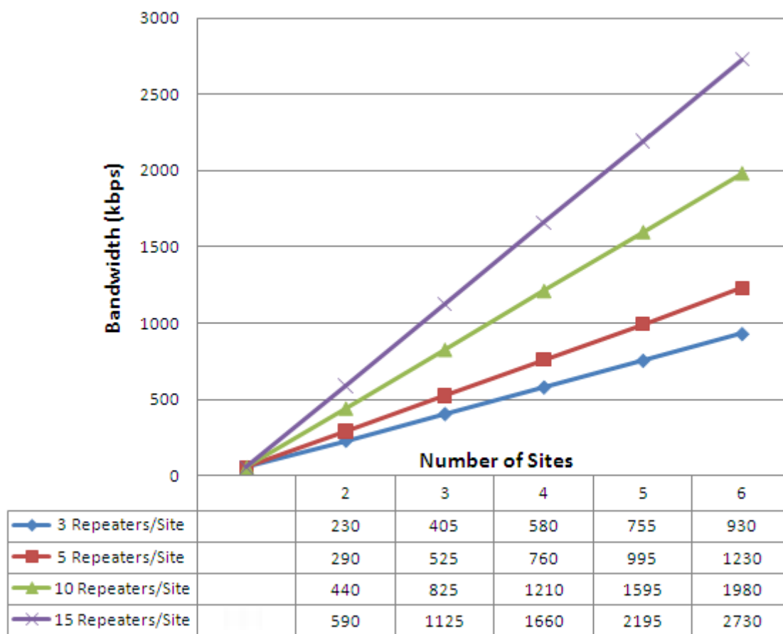
Figure 4-8 WAN Bandwidth Requirements for Multisite System (no VPN)
