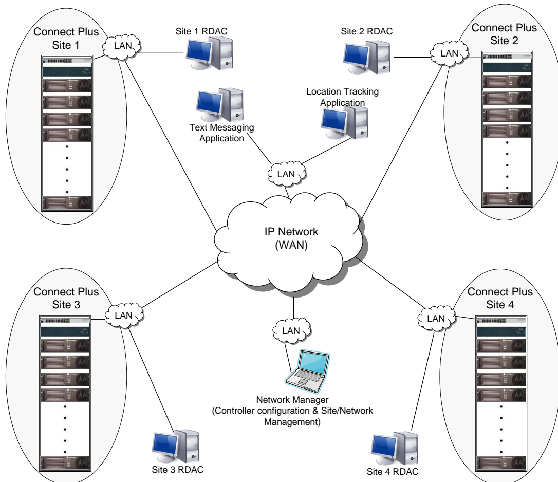
Figure 3-4 Connect Plus Multisite Configuration
