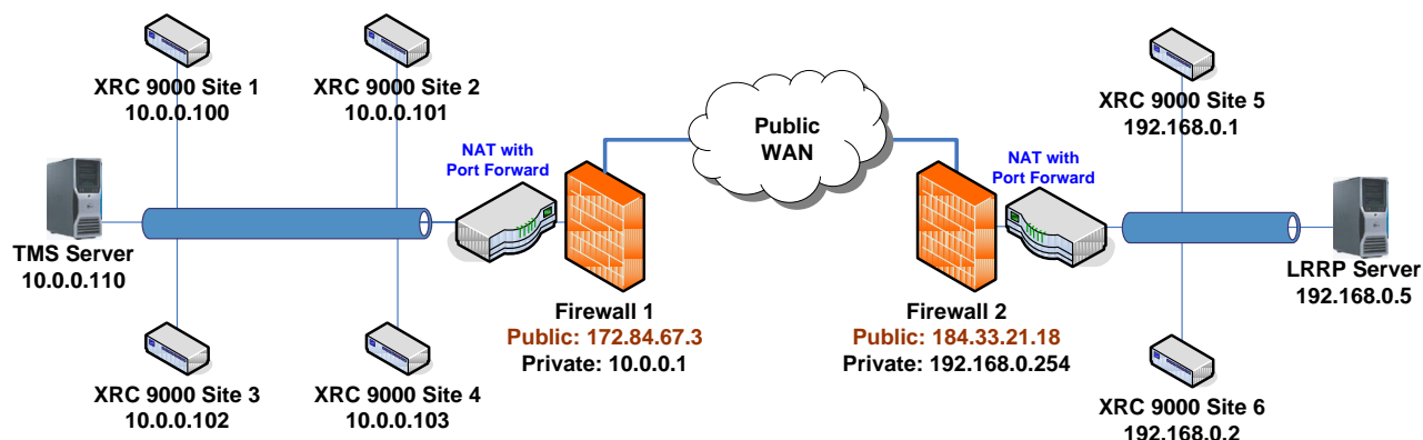
Figure 4-9 Example System IP Plan
